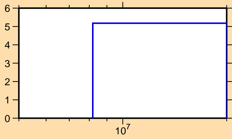
\Delta\sigma/\sigma vs. E for ^{163}\text{Lu}(n,\text{el.})
