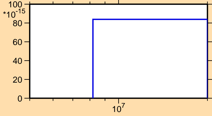
\sigma vs. E for ^{163}\text{Lu}(n,\text{pt})
