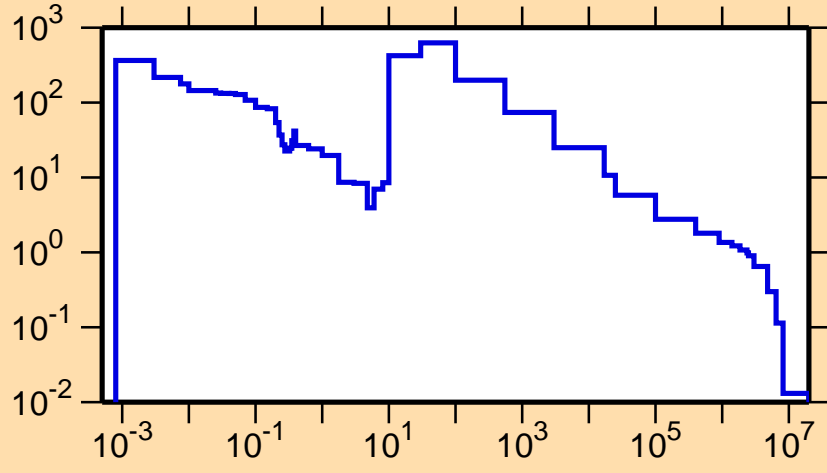
\sigma vs. E for ^{163}\text{Lu}(n,\gamma)
