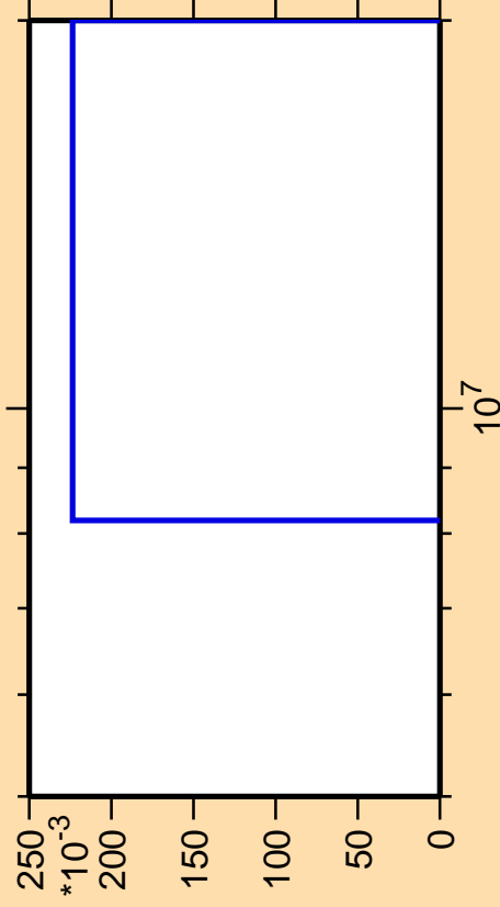
\Delta\sigma/\sigma vs. E for ^{163}\text{Lu} (mt 34)
