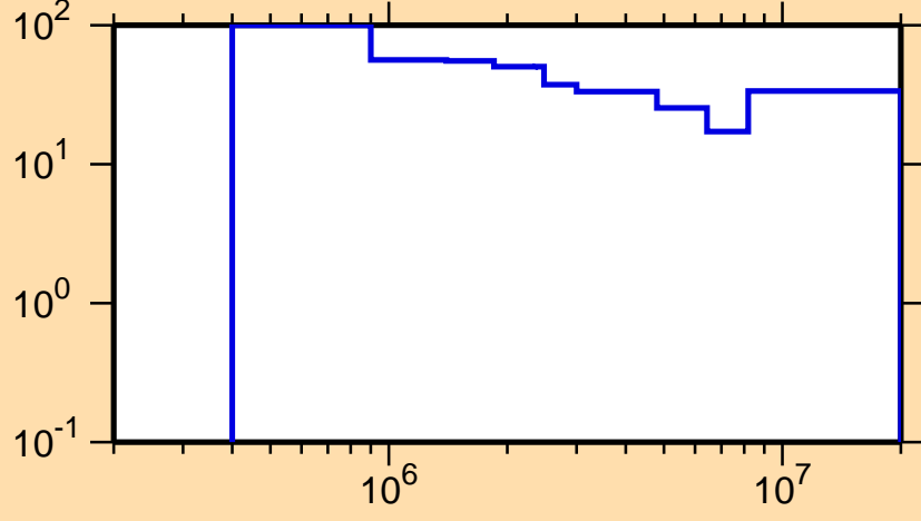
\Delta\sigma/\sigma vs. E for ^{163}\text{Lu}(n,n\text{cont.})
