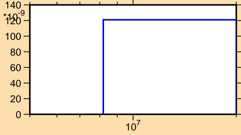
\sigma vs. E for ^{163}\text{Lu} (mt 45)
