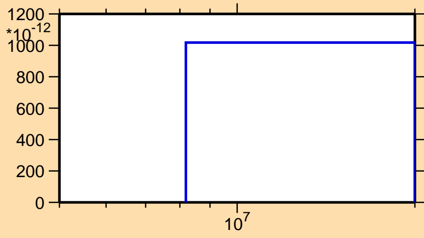
\sigma vs. E for ^{163}\text{Lu}(\text{mt117})
