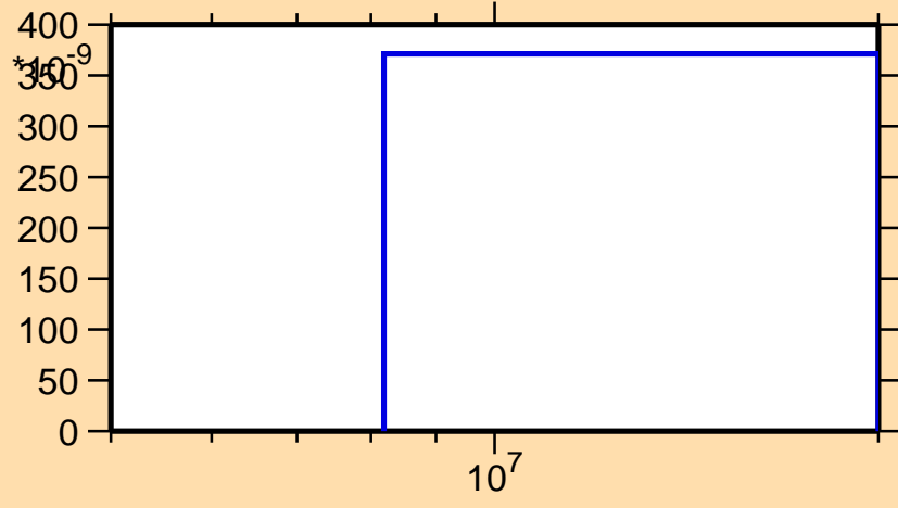
\sigma vs. E for ^{163}\text{Lu}(n,\text{He3})
