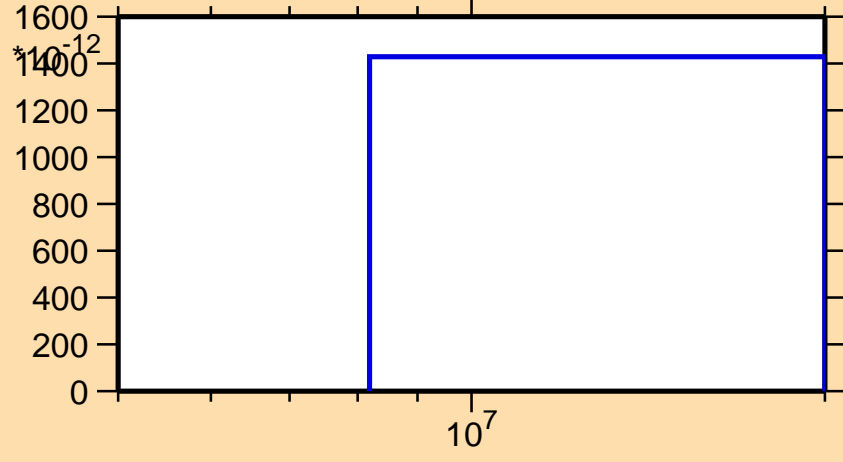
\sigma vs. E for ^{163}\text{Lu}(n,pd)
