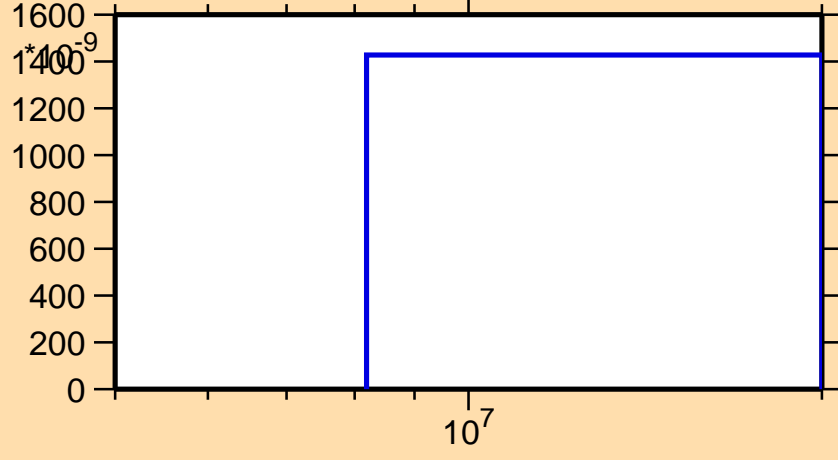
\sigma vs. E for ^{163}\text{Lu}(n,3n)
