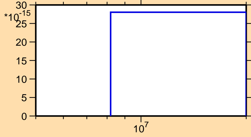
\sigma vs. E for ^{163}\text{Lu} (mt 34)
