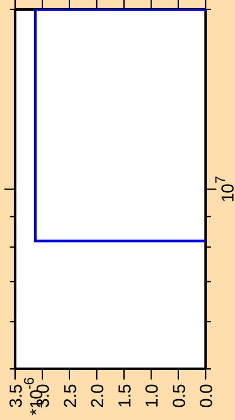
\Delta\sigma/\sigma vs. E for ^{164}\text{Lu}(\text{mt 11})
