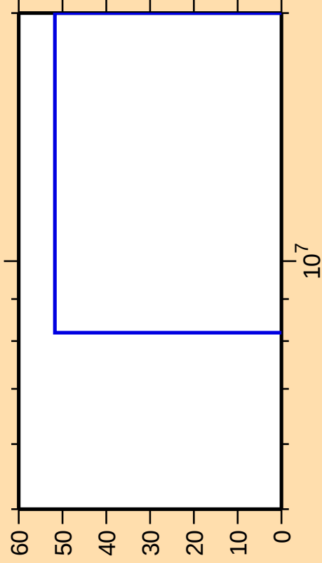
\Delta\sigma/\sigma vs. E for ^{164}\text{Lu}(\text{mt } 34)
