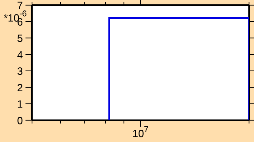
\sigma vs. E for ^{164}\text{Lu}(n,3n)
