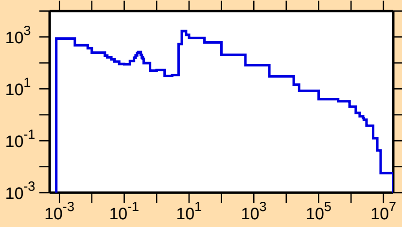
\sigma vs. E for ^{164}\text{Lu}(n,\gamma)
