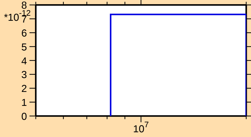
\sigma vs. E for ^{164}\text{Lu}(\text{mt } 34)
