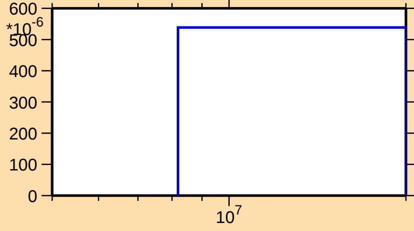
\sigma vs. E for ^{164}\text{Lu}(n,2np)
