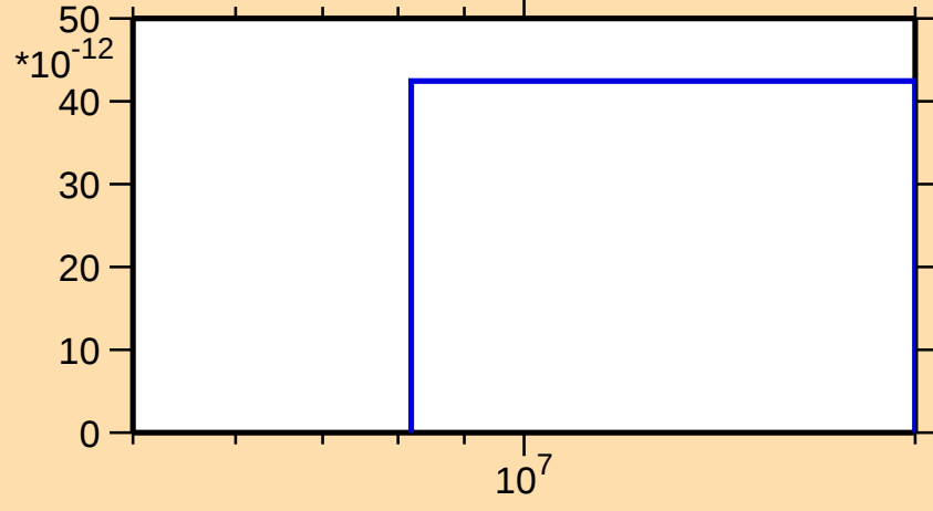
\sigma vs. E for ^{164}\text{Lu}(n,\text{pt})
