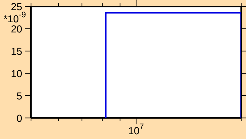
\sigma vs. E for ^{164}\text{Lu} (mt 45)
