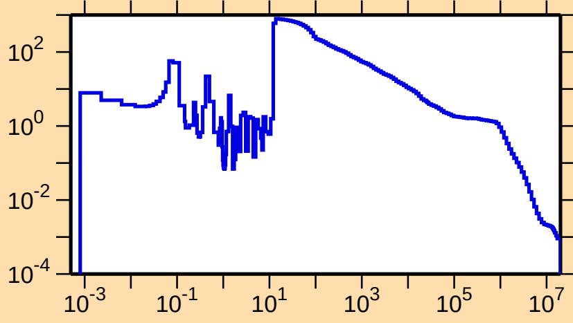
\sigma vs. E for ^{166}\text{Lu}(n,\gamma)
