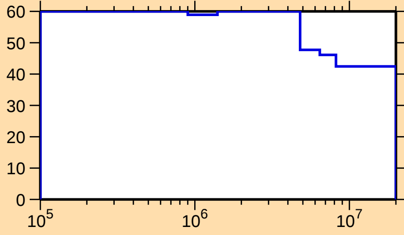
\Delta\sigma/\sigma vs. E for ^{167}\text{Lu}(n,n_1)
