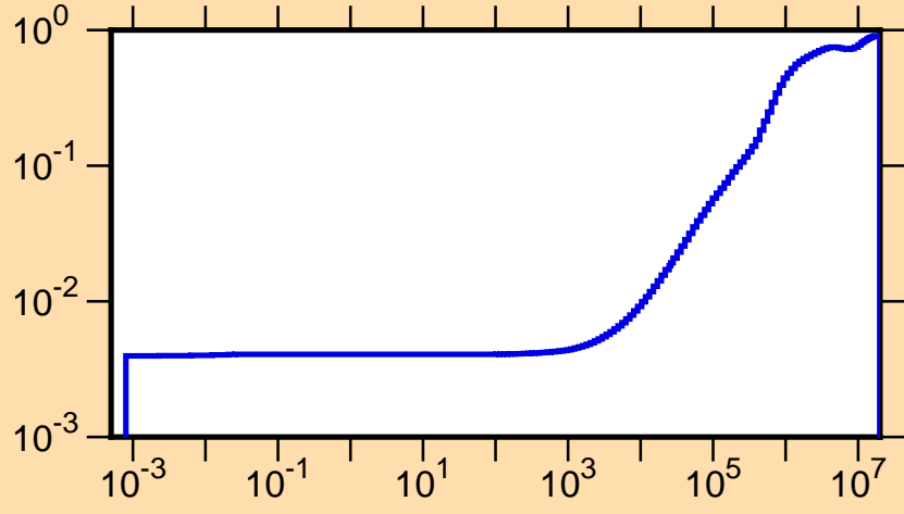
\mu vs. E for ^{170}\text{Lu}(\text{mt251})
