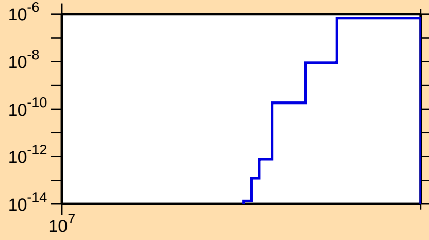
\sigma vs. E for ^{171}\text{Lu}(n,nt)
