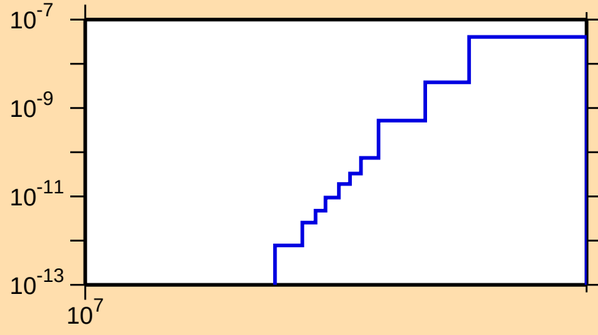
\sigma vs. E for ^{171}\text{Lu}(n,\text{He3})
