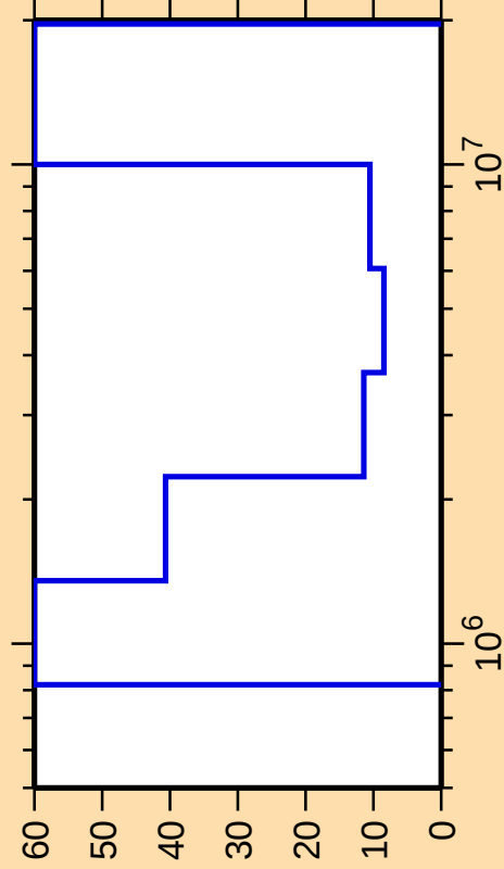
\Delta\sigma/\sigma vs. E for ^{173}\text{Lu}(n,\text{ncont.})
