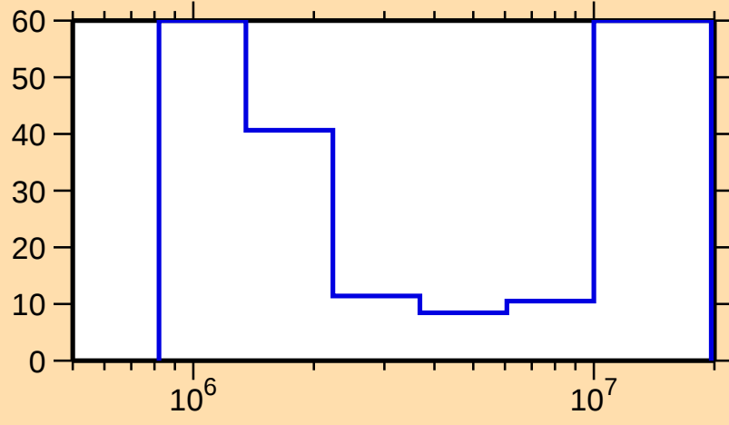
\Delta\sigma/\sigma vs. E for ^{173}\text{Lu}(n,n\text{cont.})
