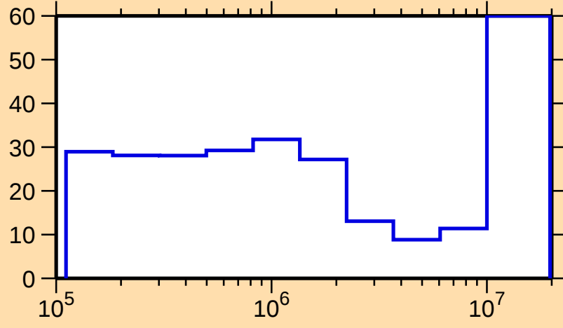
\Delta\sigma/\sigma vs. E for ^{173}\text{Lu}(n,\text{inel.})
