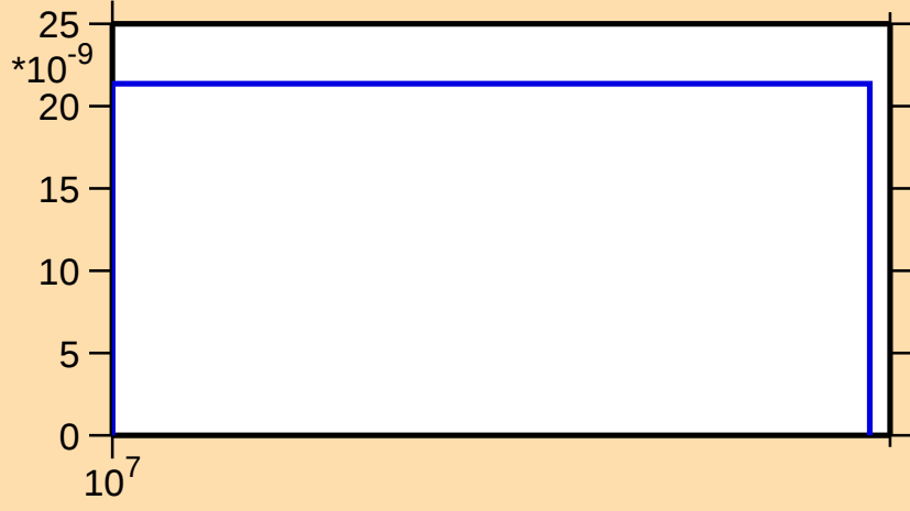
\sigma vs. E for ^{173}\text{Lu}(n,2np)
