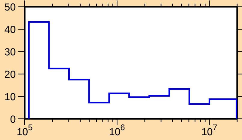
\Delta\sigma/\sigma vs. E for ^{173}\text{Lu}(n,\text{el.})
