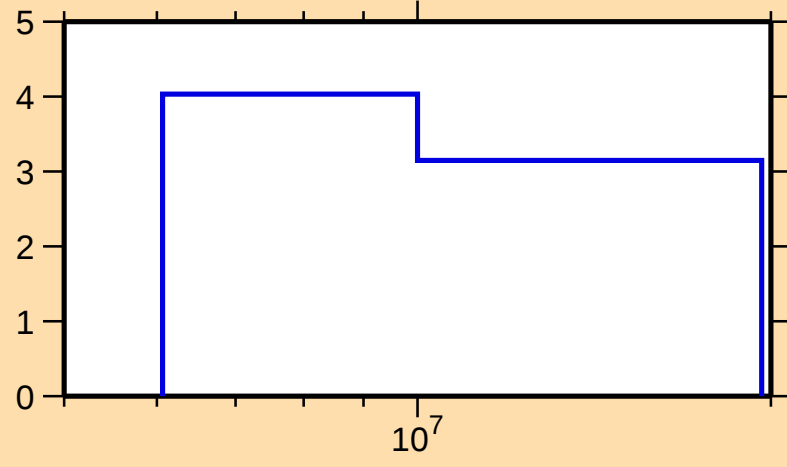
\Delta\sigma/\sigma vs. E for ^{173}\text{Lu}(n,\text{tot.})
