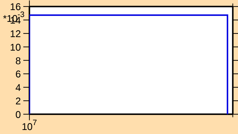
\sigma vs. E for ^{173}\text{Lu}(n,3n)
