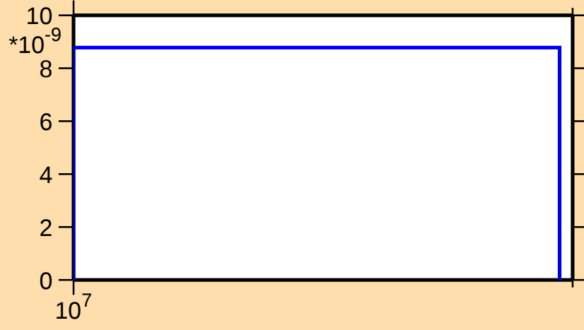
\sigma vs. E for ^{173}\text{Lu}(n,2n\alpha)
