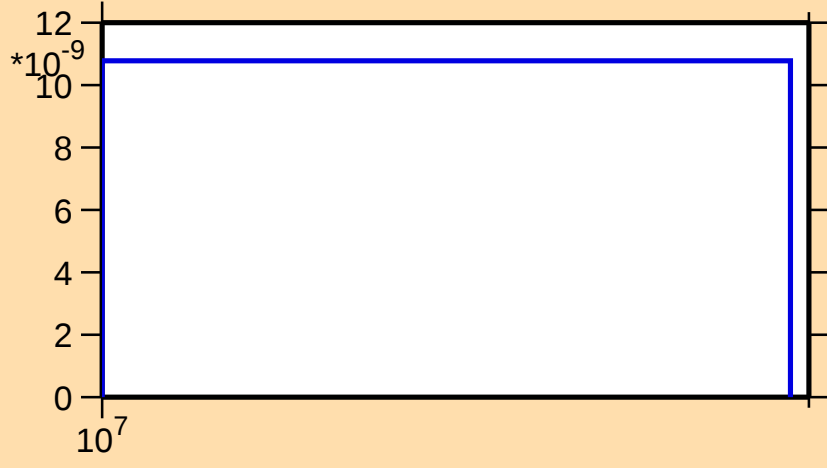
\sigma vs. E for ^{173}\text{Lu}(n,nt)
