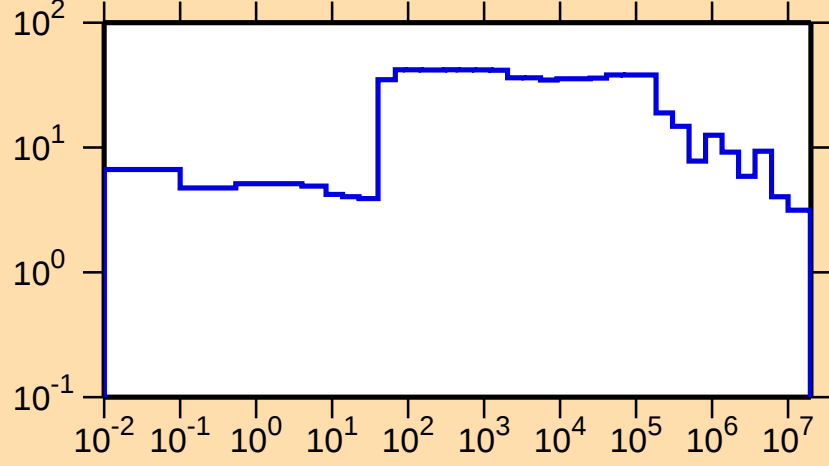
\Delta\sigma/\sigma vs. E for ^{173}\text{Lu}(n,tot.)
