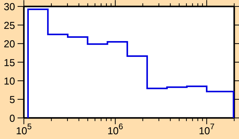
\Delta\sigma/\sigma vs. E for ^{173}\text{Lu}(n,\text{nonel.})
