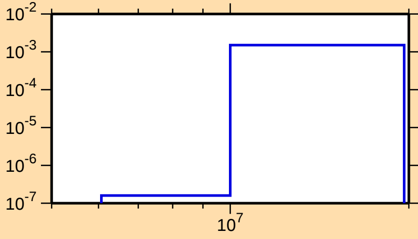
\sigma vs. E for ^{173}\text{Lu}(n,np)
