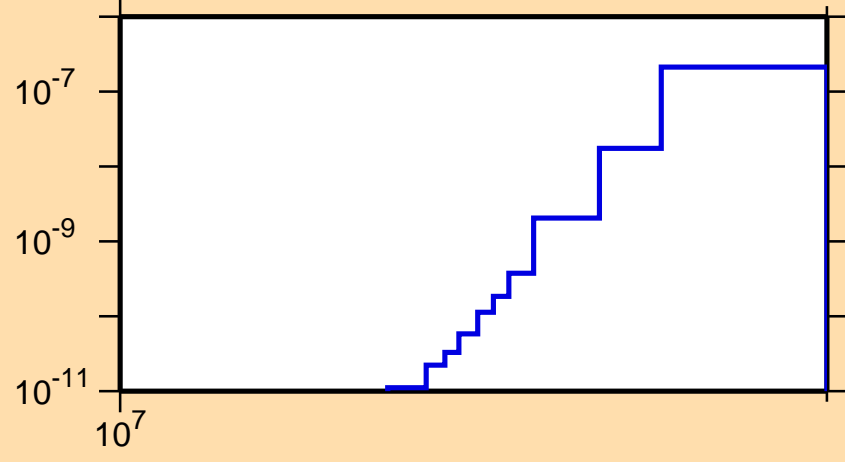
\sigma vs. E for ^{180}\text{Lu}(n,2n\alpha)
