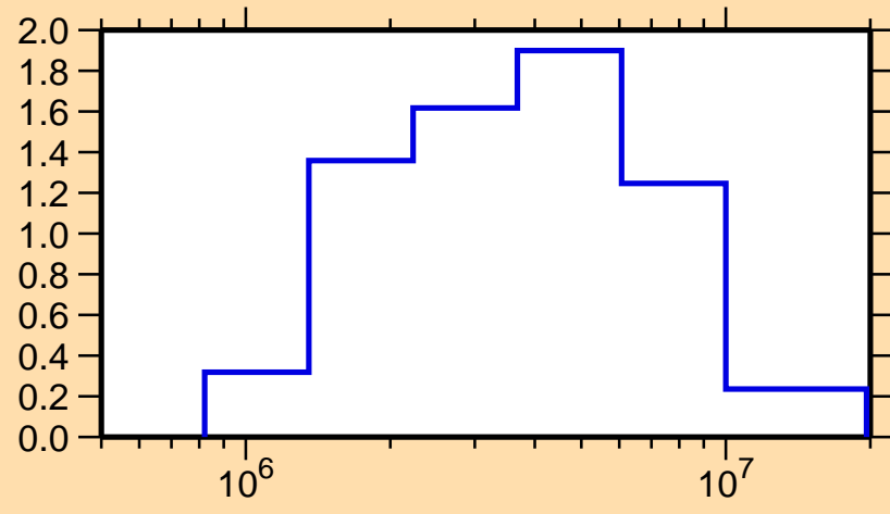
\sigma vs. E for ^{180}\text{Lu}(n,n\text{cont.})
