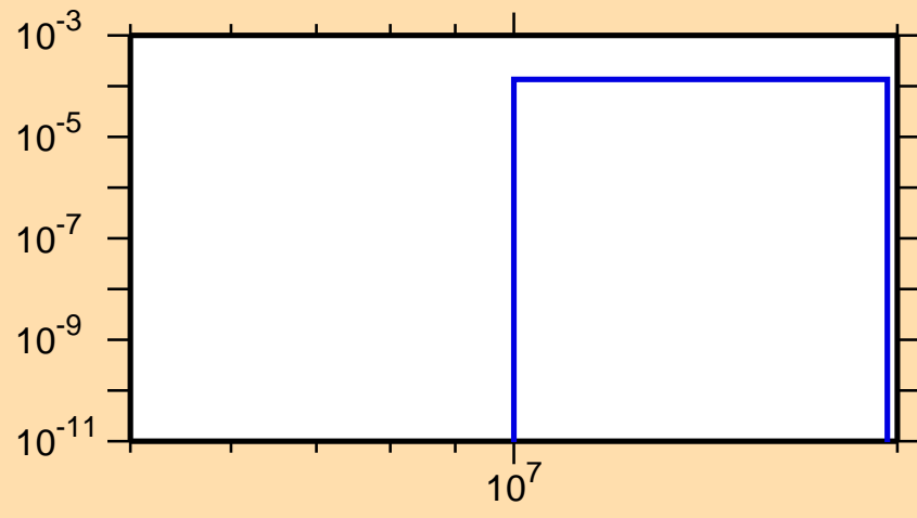
\sigma vs. E for ^{180}\text{Lu}(n,np)
