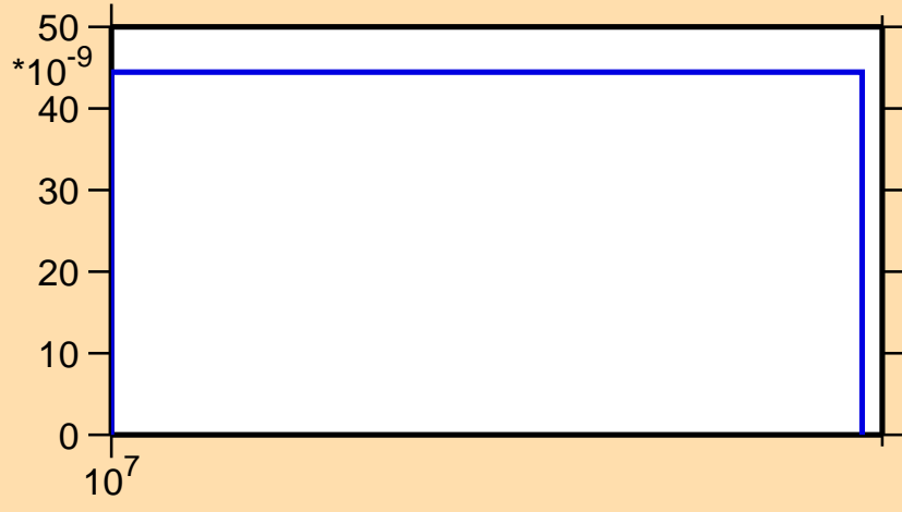
\sigma vs. E for ^{180}\text{Lu}(n,nt)
