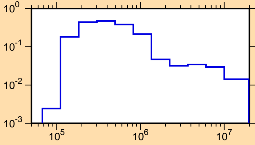
\sigma vs. E for ^{180}\text{Lu}(n,n_2)
