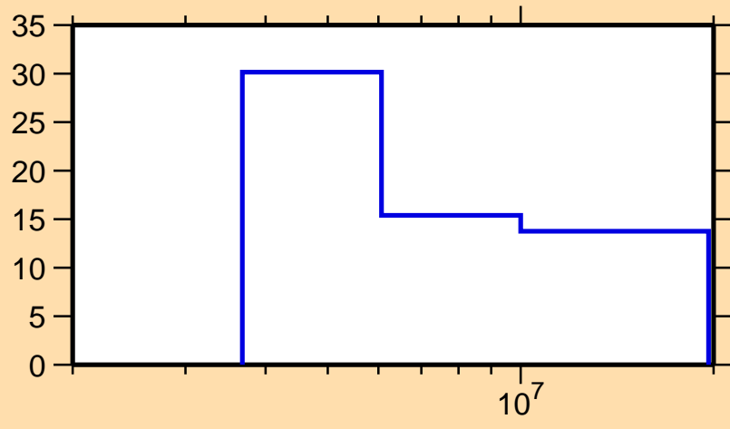
\Delta\sigma/\sigma vs. E for ^{180}\text{Lu}(n,2n)
