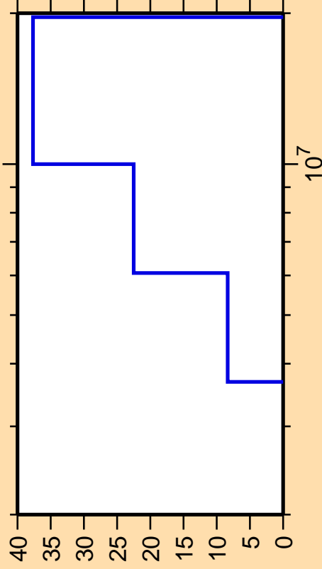
\Delta\sigma/\sigma vs. E for ^{180}\text{Lu}(n,n\text{cont.})
