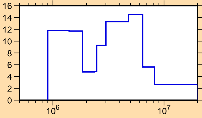
\Delta\sigma/\sigma vs. E for ^{180}\text{Lu}(n, el.)
