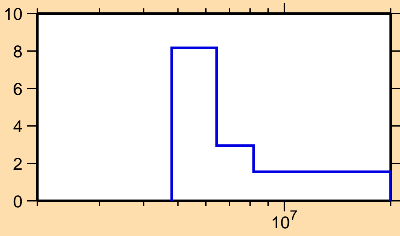
\Delta\sigma/\sigma vs. E for ^{180}\text{Lu}(n,\text{tot.})
