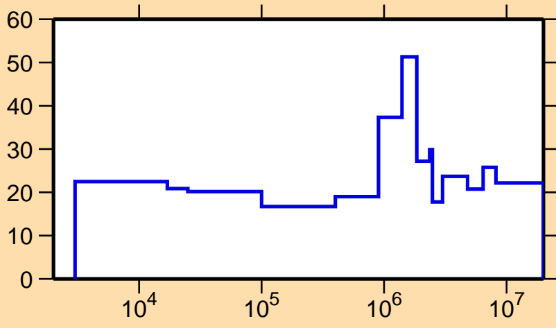
\Delta\sigma/\sigma vs. E for ^{180}\text{Lu}(n,n_1)
