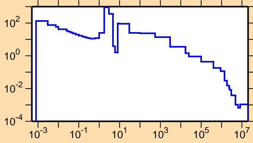
\sigma vs. E for ^{180}\text{Lu}(n,\gamma)
