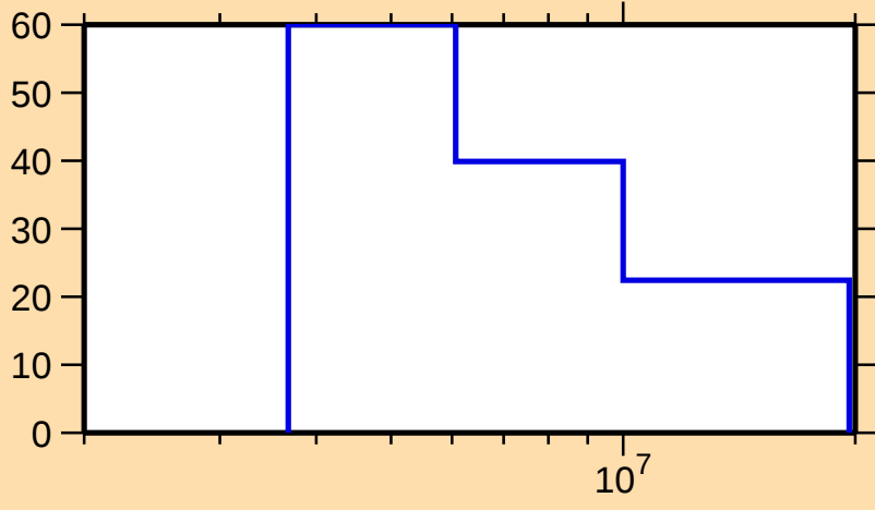
\Delta\sigma/\sigma vs. E for ^{183}\text{Lu}(n,2n)
