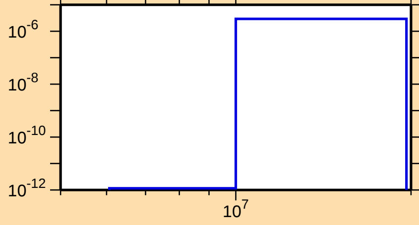
\sigma vs. E for ^{183}\text{Lu}(n,n\alpha)
