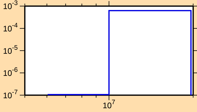
\sigma vs. E for ^{183}\text{Lu}(n,p)
