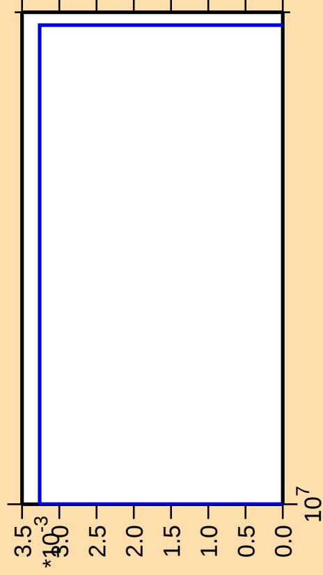
\Delta\sigma/\sigma vs. E for ^{183}\text{Lu} (mt 11)
