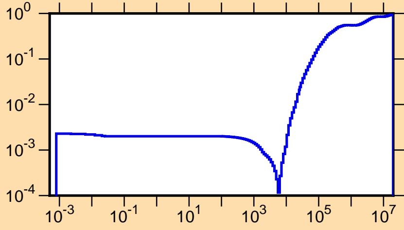
\mu vs. E for ^{291}
