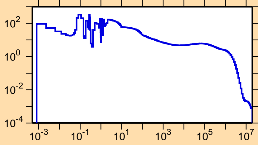
\sigma vs. E for ^{291}\gamma
