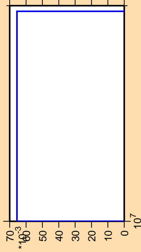
\Delta\sigma/\sigma vs. E for ^{291}
