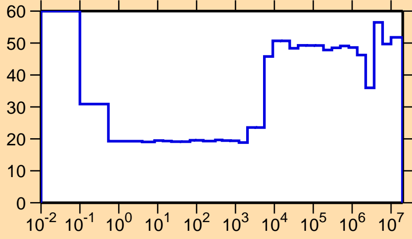
\Delta\sigma/\sigma vs. E for ^{291}\gamma
