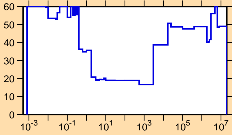
\Delta\sigma/\sigma vs. E for ^{291}\text{Pb}
