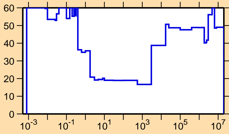
\Delta\sigma/\sigma vs. E for ^{291}\gamma
