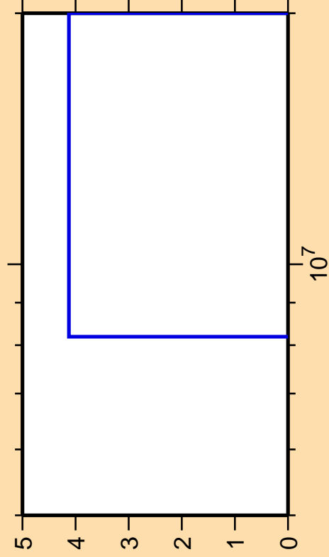
\Delta\sigma/\sigma vs. E for 291
