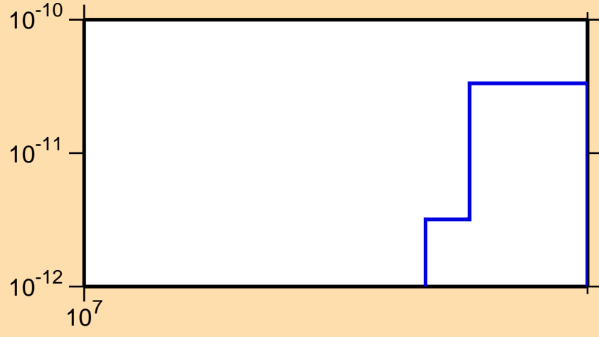
\sigma vs. E for ^{246}\text{Md}(n,\text{pt})
