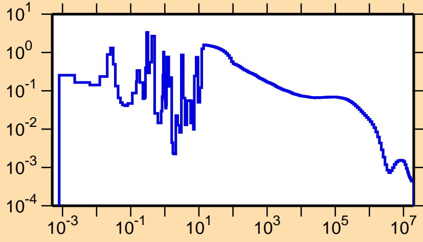
\sigma vs. E for ^{246}\text{Md}(n,\gamma)
