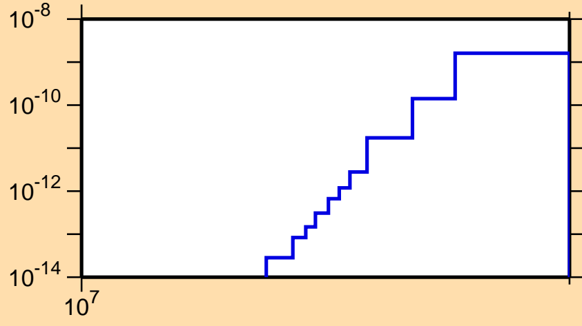
\sigma vs. E for ^{246}\text{Md} (mt 34)
