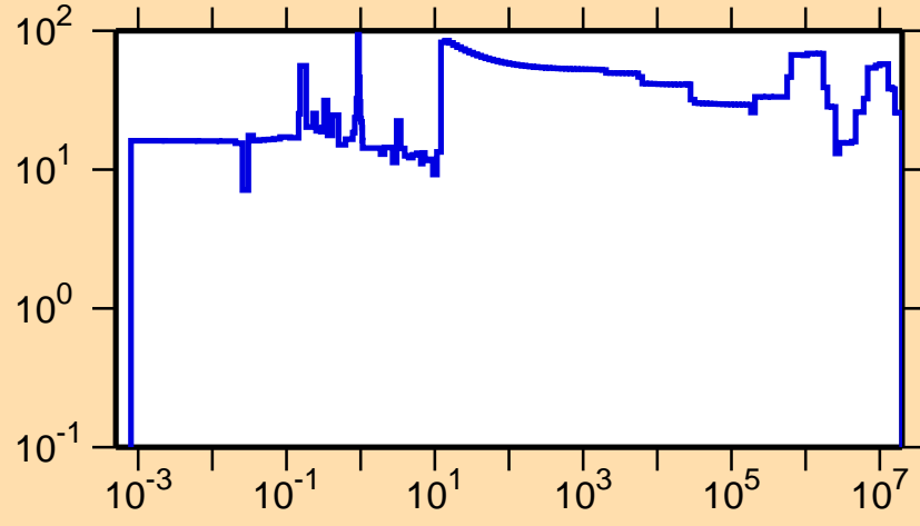
\Delta\sigma/\sigma vs. E for ^{246}\text{Md}(n,el.)
