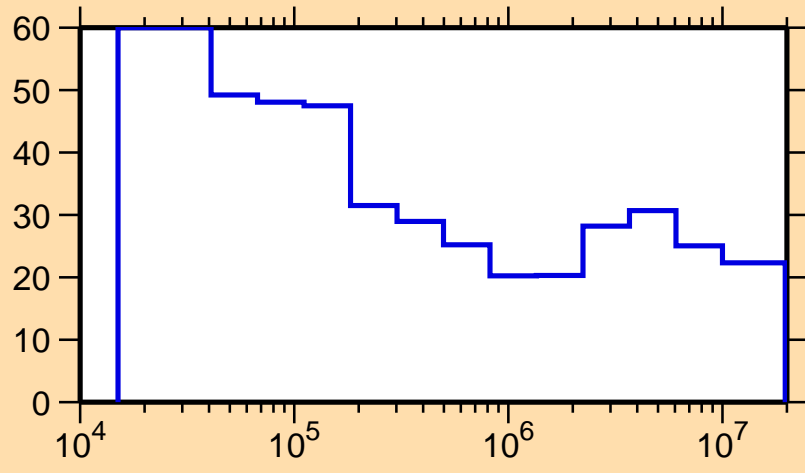
\Delta\sigma/\sigma vs. E for ^{246}\text{Md}(n,n\text{onel.})
