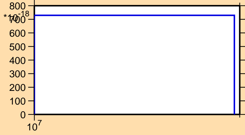
\sigma vs. E for ^{246}\text{Md} (mt 42)
