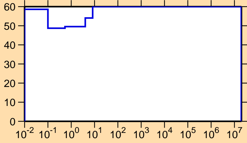
\Delta\sigma/\sigma vs. E for ^{246}\text{Md}(n,\gamma)
