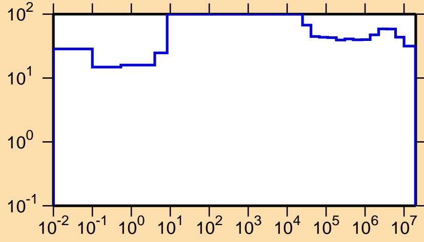
\Delta\sigma/\sigma vs. E for ^{246}\text{Md}(n,f)
