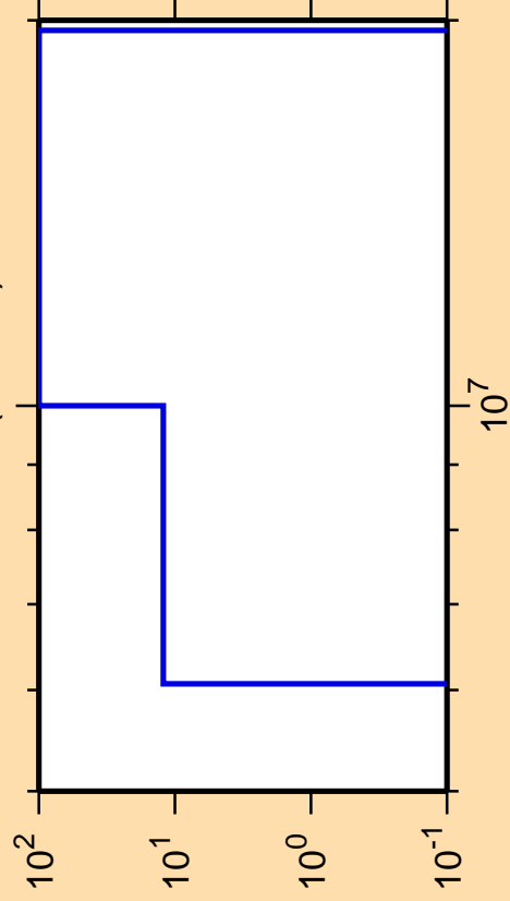
\Delta\sigma/\sigma vs. E for ^{246}\text{Md}(n,\text{He3})
