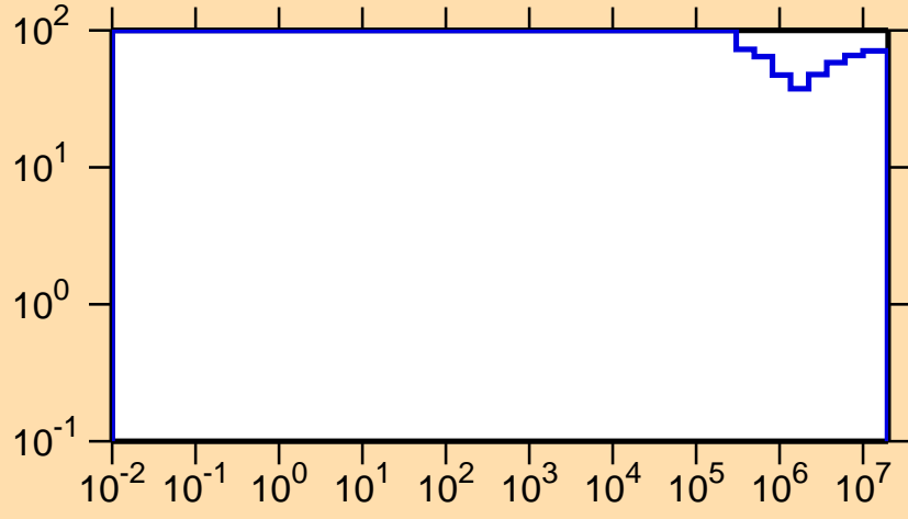
\Delta\sigma/\sigma vs. E for ^{246}\text{Md}(n,p)
