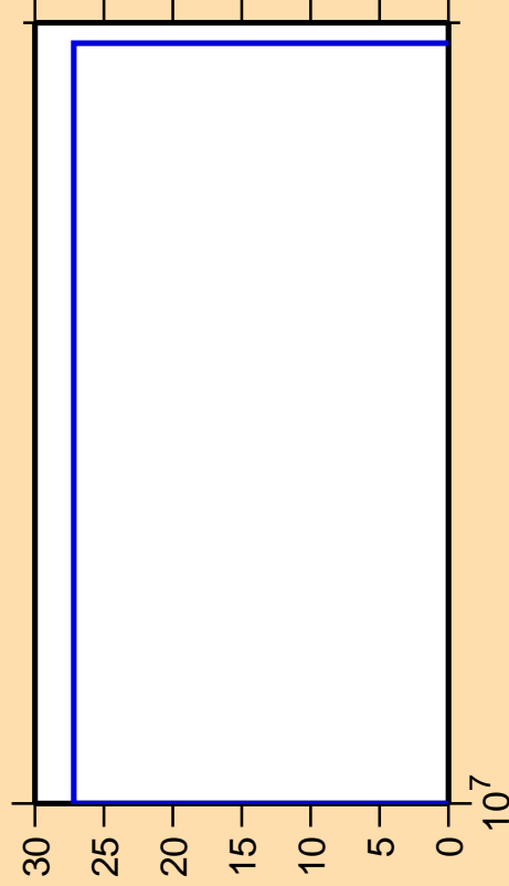
\Delta\sigma/\sigma vs. E for ^{246}\text{Md}(n,\text{pd})
