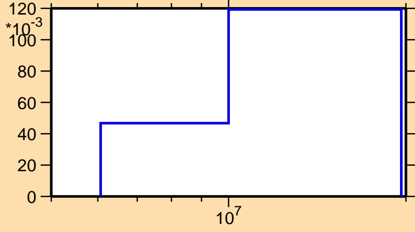
\sigma vs. E for ^{246}\text{Md}(n,2n)
