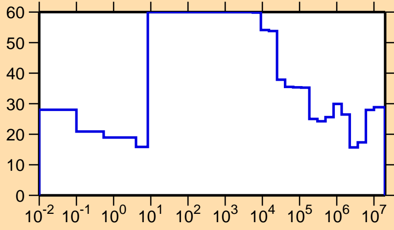
\Delta\sigma/\sigma vs. E for ^{246}\text{Md}(n,\text{tot.})
