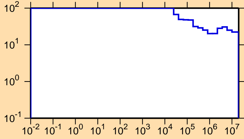
\Delta\sigma/\sigma vs. E for ^{246}\text{Md}(n,\text{nonel.})
