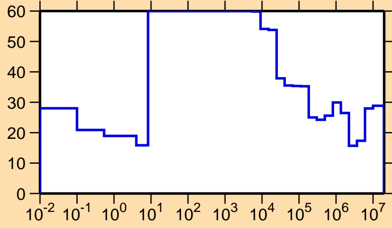
\Delta\sigma/\sigma vs. E for ^{246}\text{Md}(n,\text{tot.})
