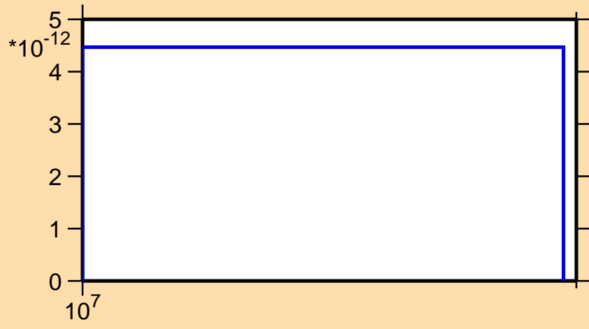
\sigma vs. E for ^{246}\text{Md}(n,\text{pd})
