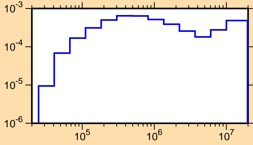
\sigma vs. E for ^{246}\text{Md}(n,n\alpha)
