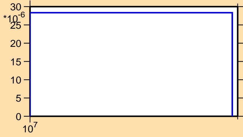
\sigma vs. E for ^{246}\text{Md}(n,3n)
