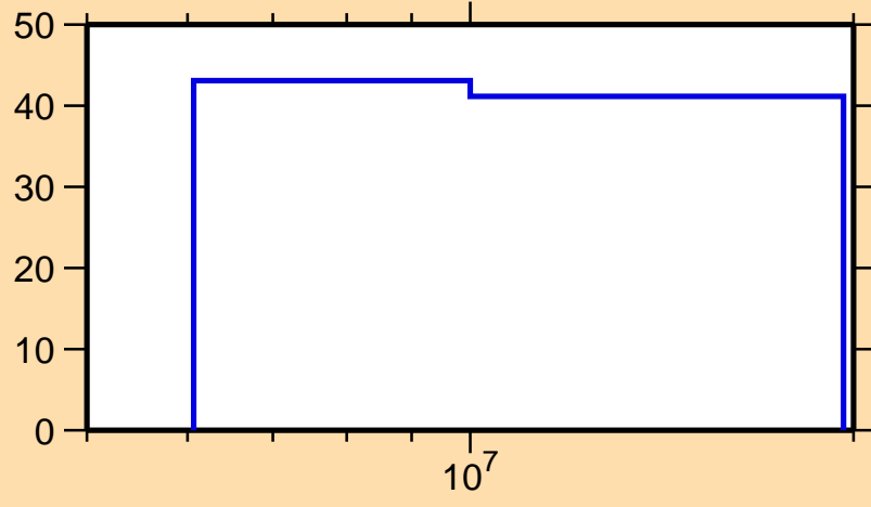
\Delta\sigma/\sigma vs. E for ^{246}\text{Md}(n,\text{el.})
