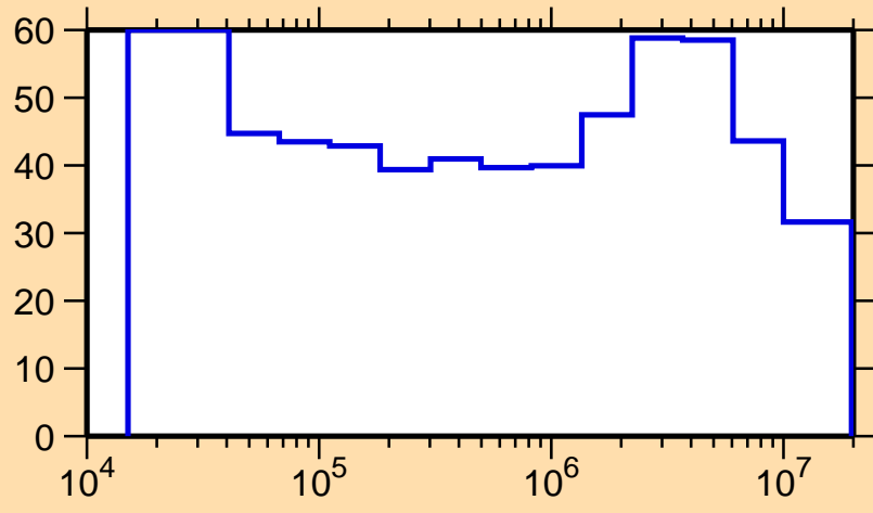
\Delta\sigma/\sigma vs. E for ^{246}\text{Md}(n,f)
