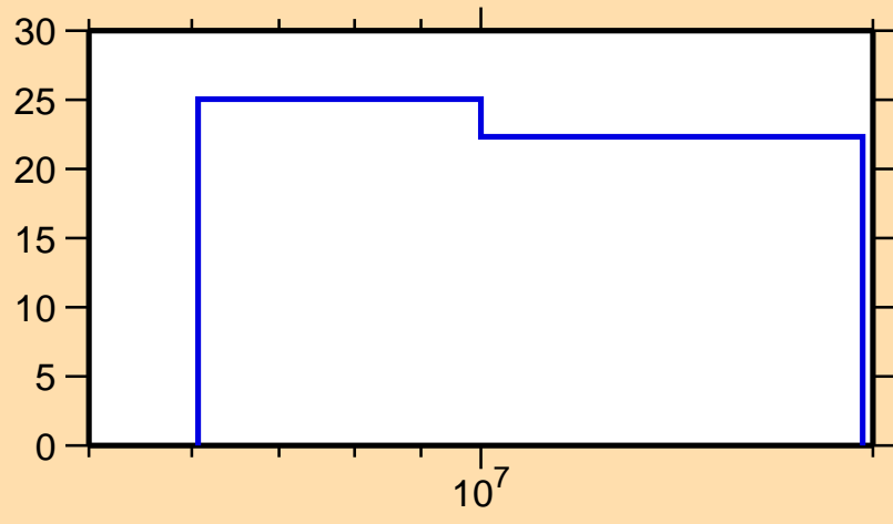
\Delta\sigma/\sigma vs. E for ^{246}\text{Md}(n,\text{nonel.})
