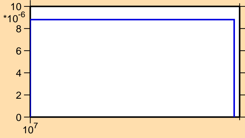
\sigma vs. E for ^{246}\text{Md}(n,3n\alpha)
