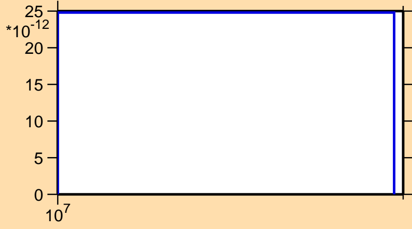
\sigma vs. E for ^{246}\text{Md} (mt 34)
