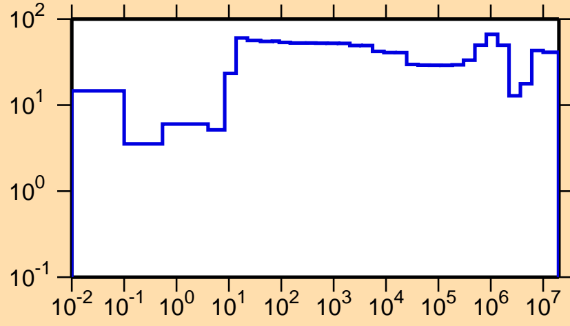
\Delta\sigma/\sigma vs. E for ^{246}\text{Md}(n,\text{el.})
