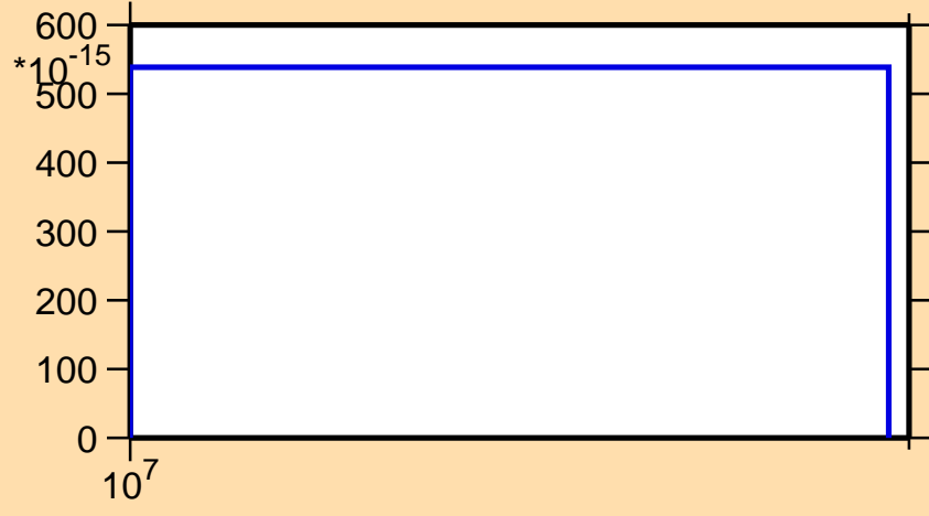
\sigma vs. E for ^{246}\text{Md}(n,\text{pt})
