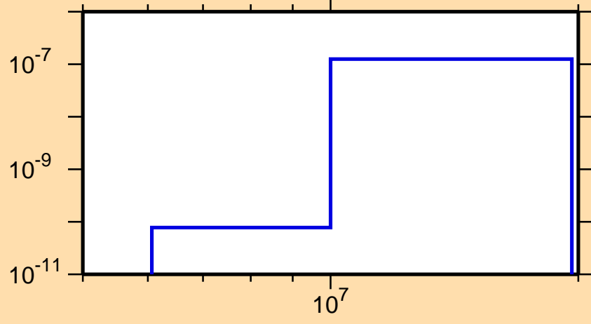
\sigma vs. E for ^{246}\text{Md}(\text{mt117})
