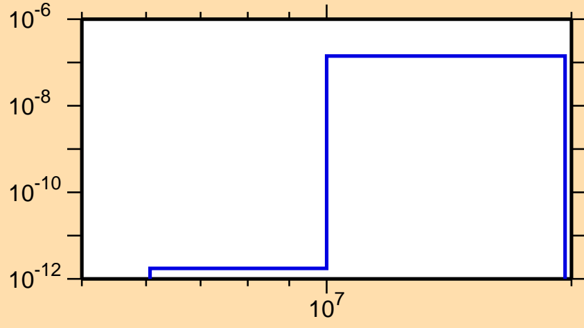
\sigma vs. E for ^{246}\text{Md}(n,\text{He3})
