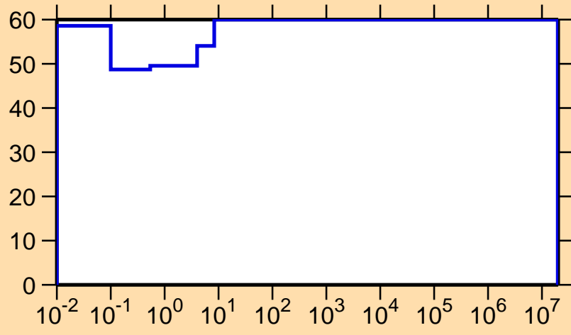
\Delta\sigma/\sigma vs. E for ^{246}\text{Md}(n,\gamma)
