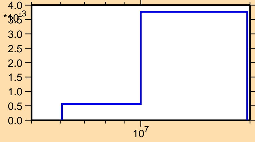
\sigma vs. E for ^{246}\text{Md}(n,2n\alpha)
