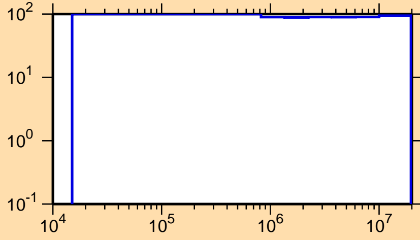
\Delta\sigma/\sigma vs. E for ^{246}\text{Md}(n,n\text{cont.})
