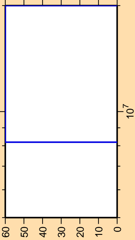
\Delta\sigma/\sigma vs. E for ^{246}\text{Md}(n,nd)
