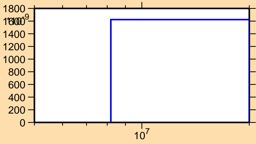
\sigma vs. E for ^{246}\text{Md}(n,nd)
