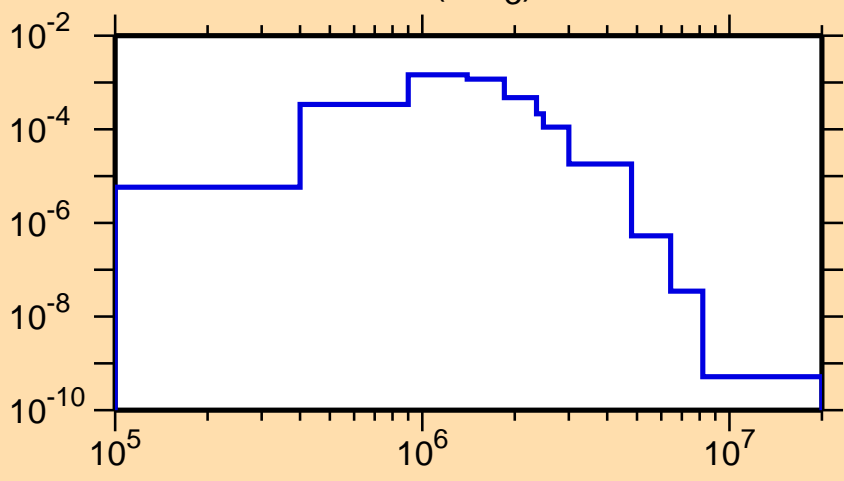
\sigma vs. E for ^{246}\text{Md}(n,n_3)
