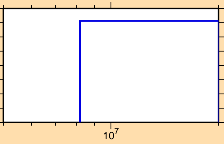
\sigma vs. E for ^{246}\text{Md}(n,3n\alpha)
