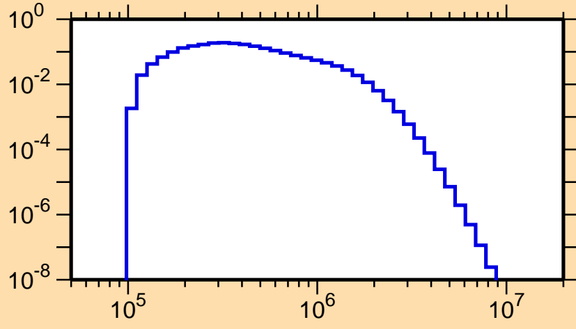
\sigma vs. E for ^{248}\text{Md}(n,n_1)
