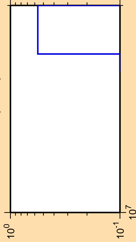
\Delta\sigma/\sigma vs. E for ^{248}\text{Md} (mt 11)
