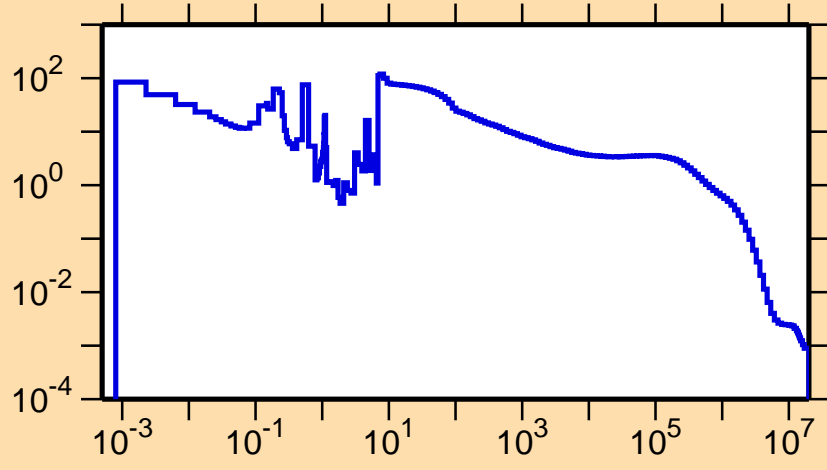
\sigma vs. E for ^{248}\text{Md}(n,\gamma)
