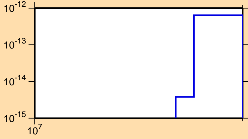
\sigma vs. E for ^{248}\text{Md} (mt 11)
