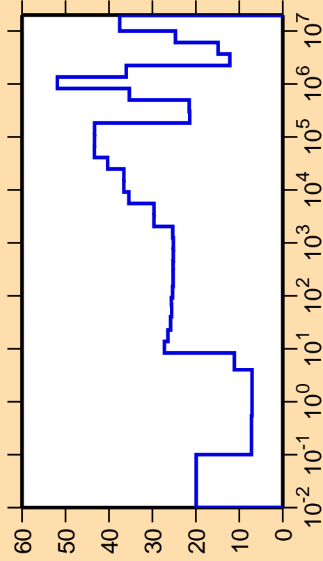
\Delta\sigma/\sigma vs. E for ^{248}\text{Md}(n,\text{el.})
