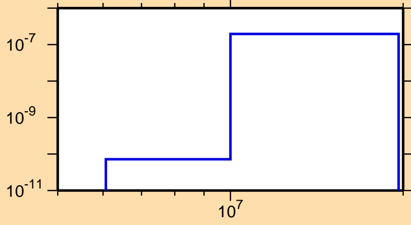
\sigma vs. E for ^{248}\text{Md}(\text{mt117})
