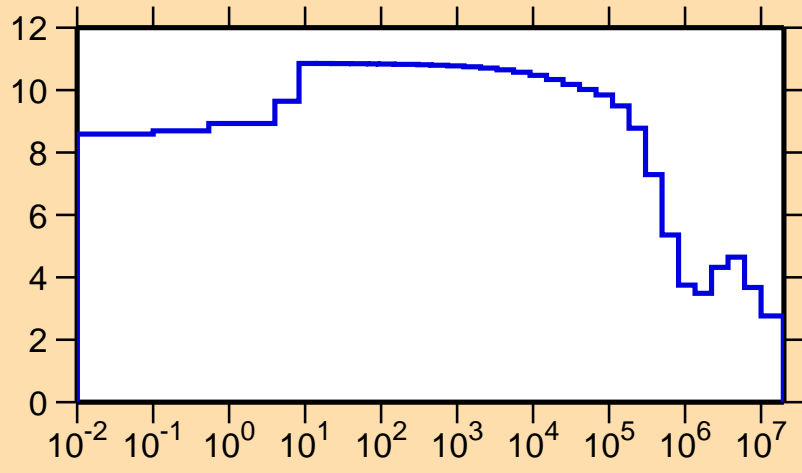
\sigma vs. E for ^{248}\text{Md}(n,\text{el.})
