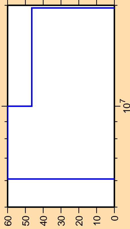
\Delta\sigma/\sigma vs. E for ^{248}\text{Md}(n,f)
