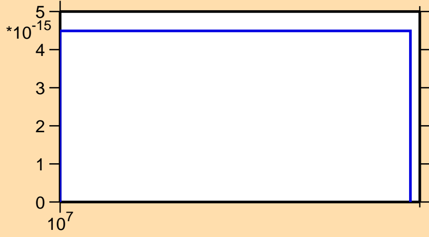
\sigma vs. E for ^{248}\text{Md}(\text{mt } 11)
