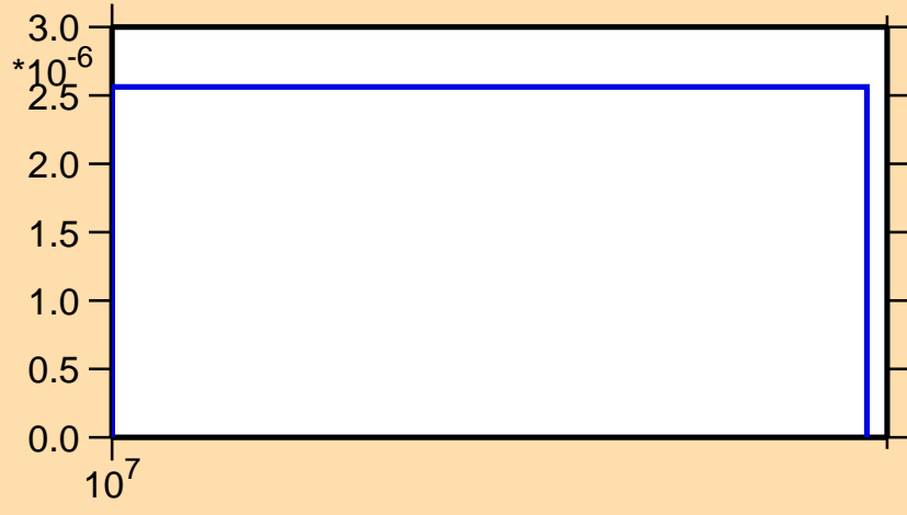
\sigma vs. E for ^{248}\text{Md}(n,3n\alpha)
