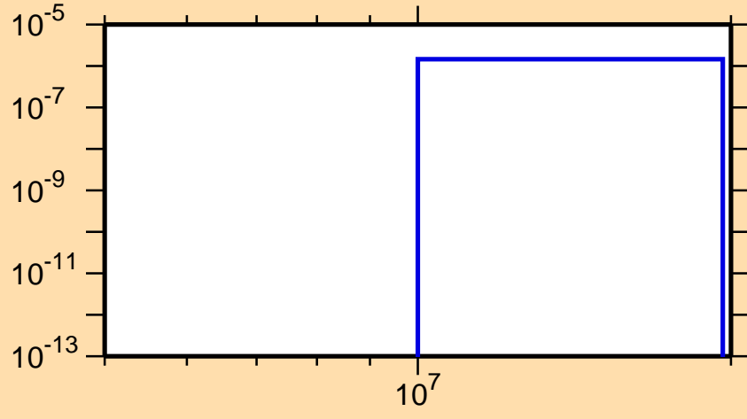
\sigma vs. E for ^{248}\text{Md}(n,nd)
