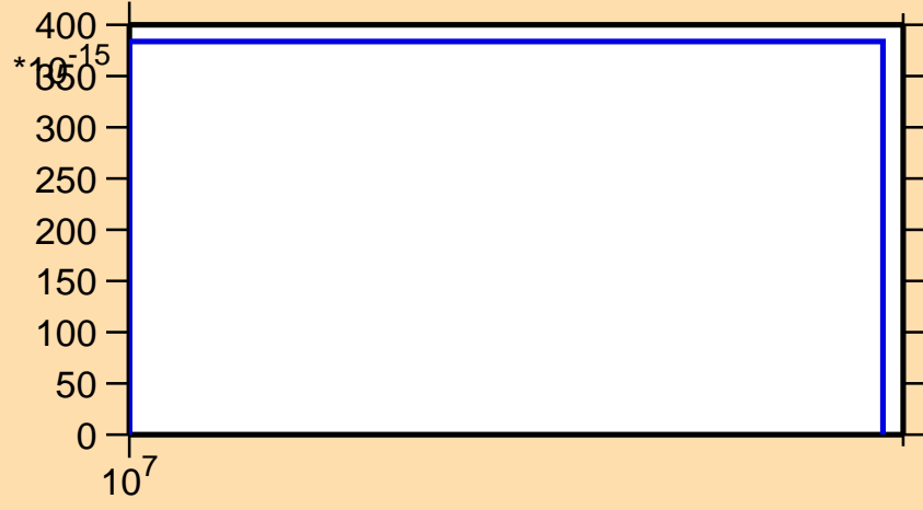
\sigma vs. E for ^{248}\text{Md}(n,\text{pd})
