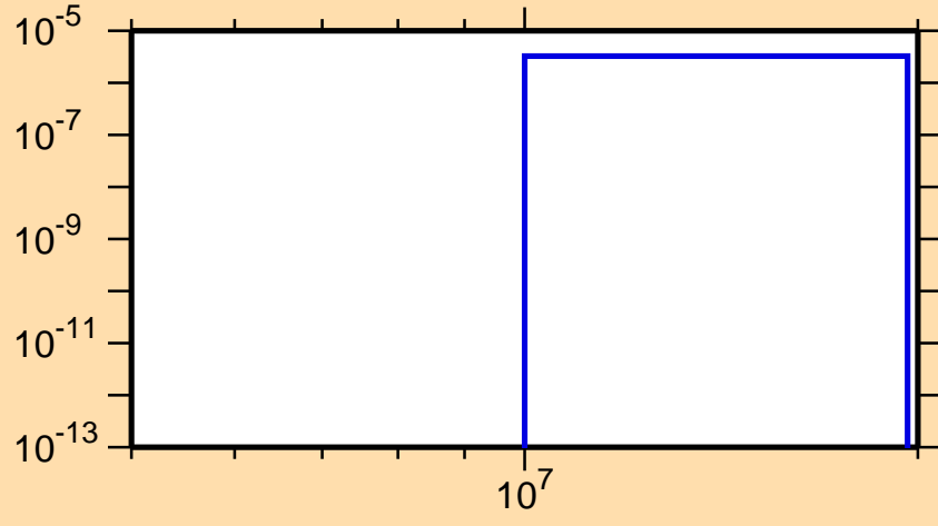
\sigma vs. E for ^{248}\text{Md}(n,2np)
