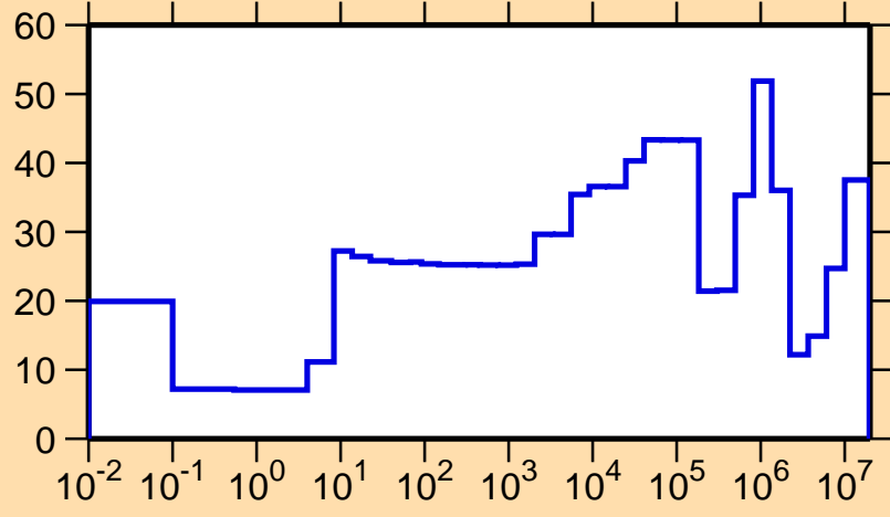
\Delta\sigma/\sigma vs. E for ^{248}\text{Md}(n,\text{el.})
