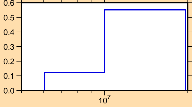
\sigma vs. E for ^{248}\text{Md}(n,2n)
