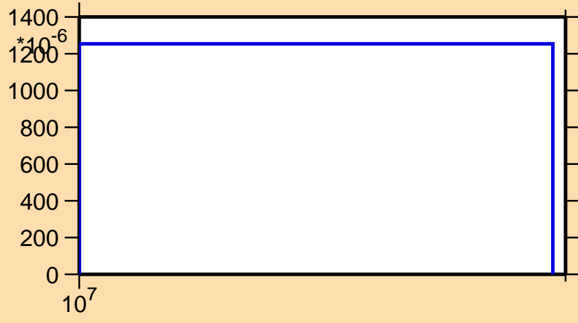
\sigma vs. E for ^{248}\text{Md}(n,3n)
