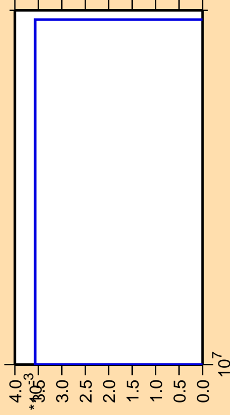
\Delta\sigma/\sigma vs. E for ^{248}\text{Md}(\text{mt } 11)
