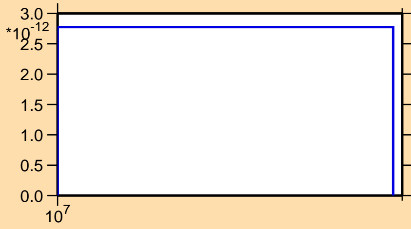
\sigma vs. E for ^{248}\text{Md} (mt 34)
