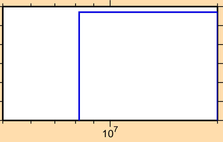
\sigma vs. E for ^{248}\text{Md}(\text{mt } 11)
