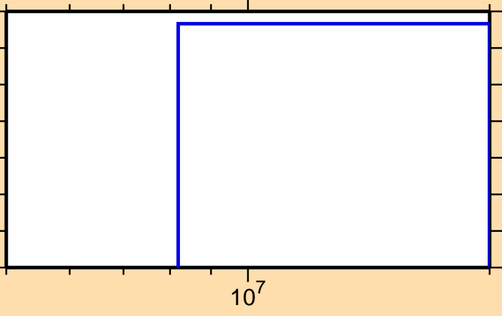
\sigma vs. E for ^{248}\text{Md}(n,nt)
