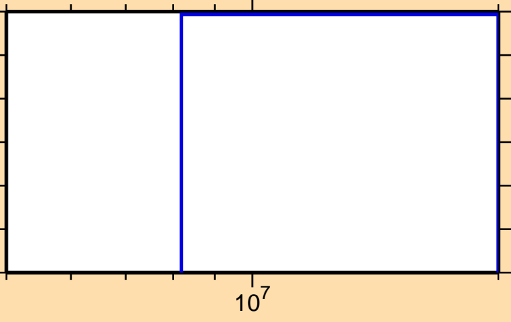
\sigma vs. E for ^{248}\text{Md}(n,nd)
