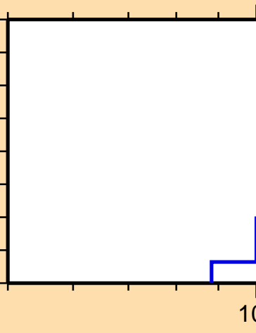
\sigma vs. E for ^{249}\text{Md}(n,\text{He3})
