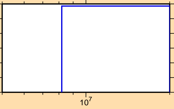
\sigma vs. E for ^{249}\text{Md}(n,\text{He3})
