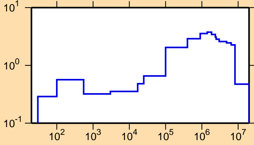
\sigma vs. E for ^{249}\text{Md}(n,\text{inel.})
