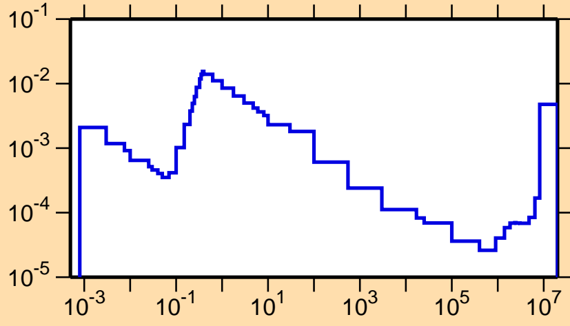
\sigma vs. E for ^{249}\text{Md}(n,\alpha)
