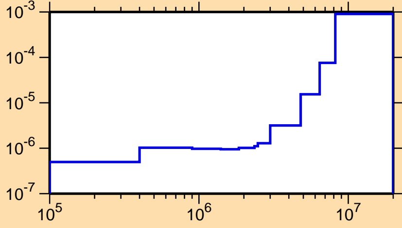
\sigma vs. E for ^{249}\text{Md}(n,n\alpha)
