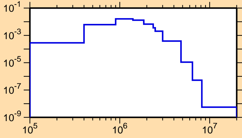
\sigma vs. E for ^{249}\text{Md}(n,n_2)
