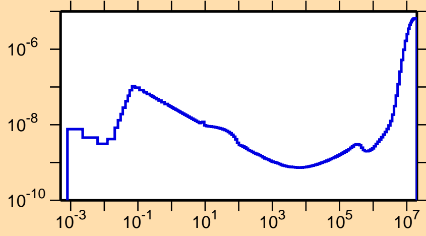
\sigma vs. E for ^{250}\text{Md}(n,p\alpha)
