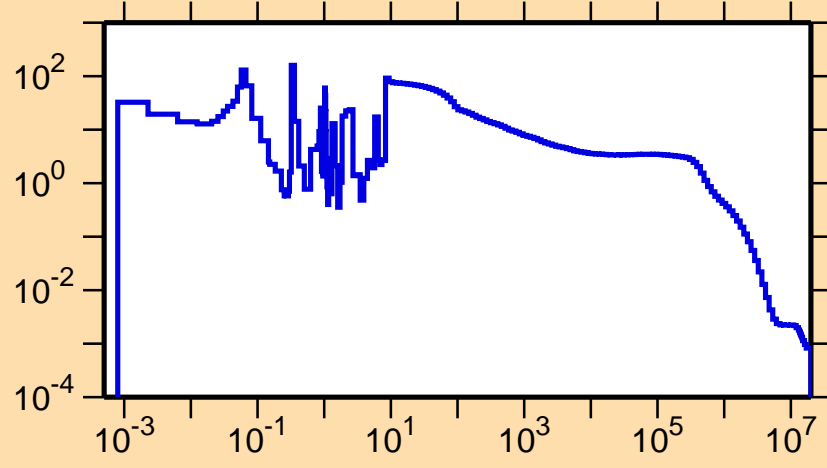
\sigma vs. E for ^{250}\text{Md}(n,\gamma)
