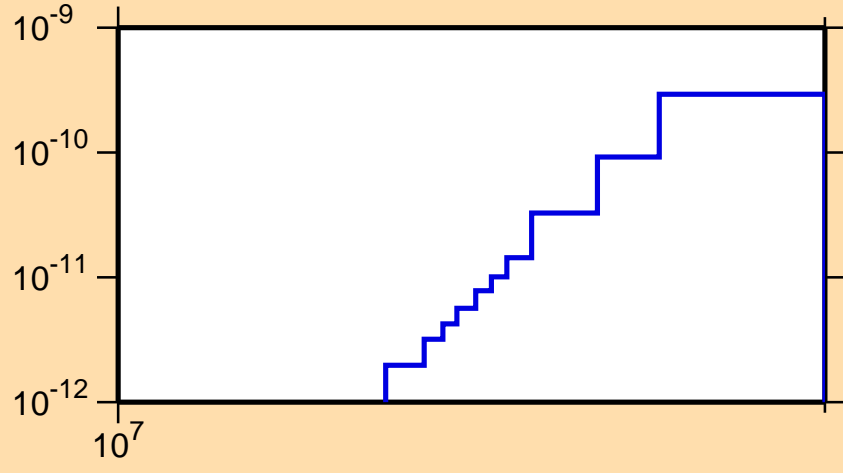
\sigma vs. E for ^{250}\text{Md} (mt 45)
