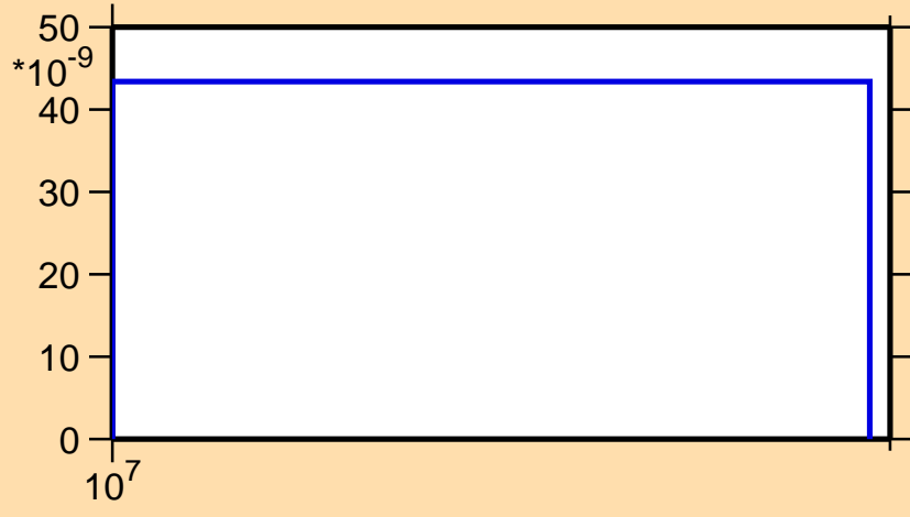
\sigma vs. E for ^{250}\text{Md}(n,nt)
