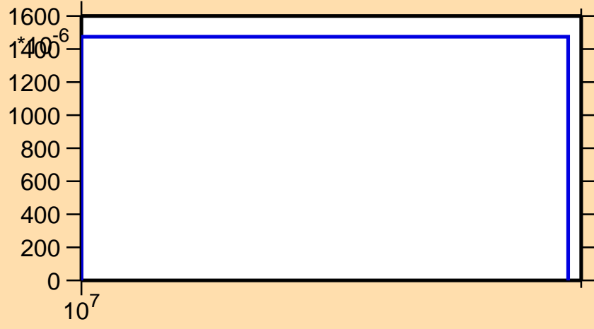
\sigma vs. E for ^{250}\text{Md}(n,3n\alpha)
