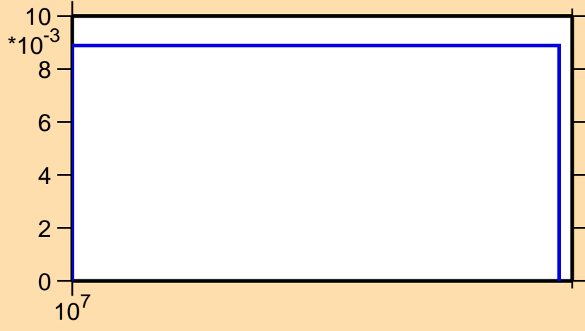
\sigma vs. E for ^{250}\text{Md}(n,3n)
