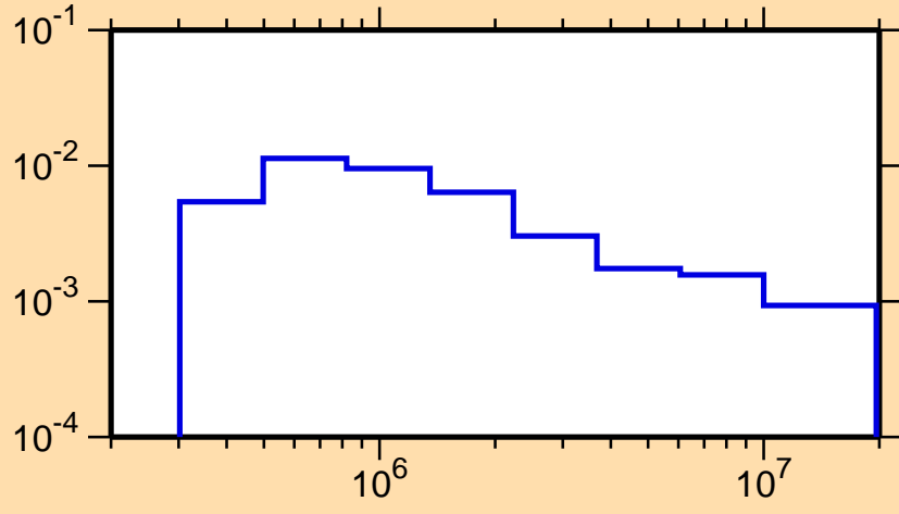
\sigma vs. E for ^{250}\text{Md}(n,n_4)
