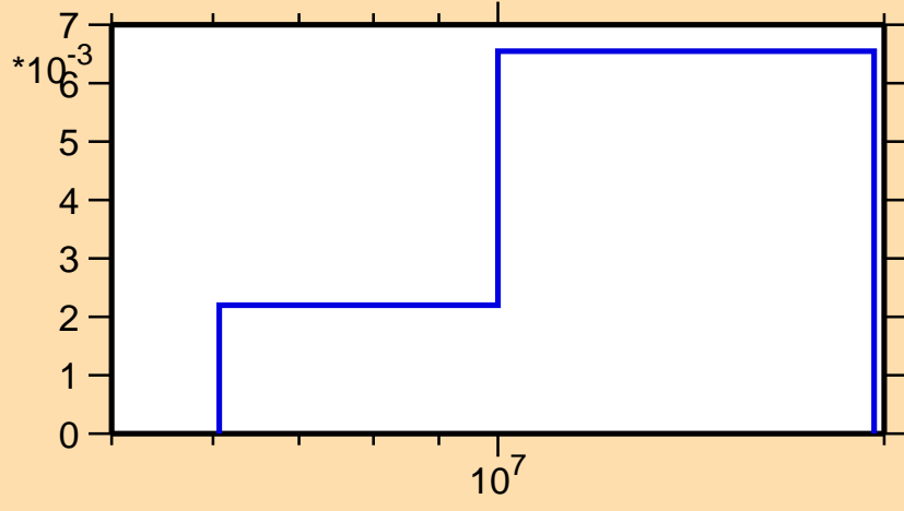
\sigma vs. E for ^{250}\text{Md}(n,2n\alpha)
