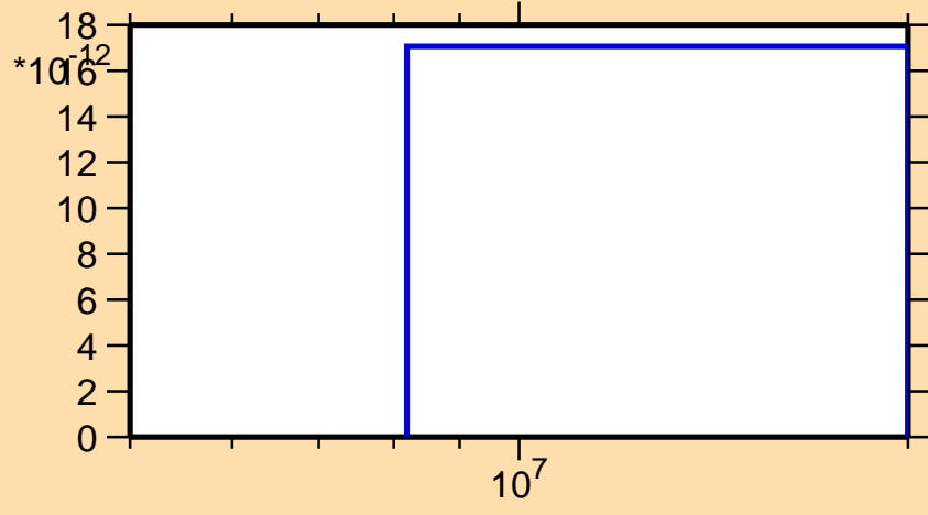
\sigma vs. E for ^{250}\text{Md}(\text{mt117})
