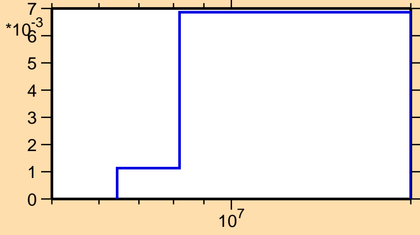
\sigma vs. E for ^{250}\text{Md}(n,2n\alpha)
