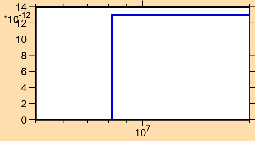
\sigma vs. E for ^{250}\text{Md}(\text{mt } 45)
