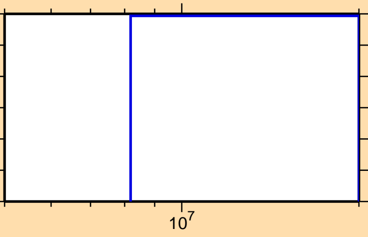
\sigma vs. E for ^{250}\text{Md}(n,3n\alpha)
