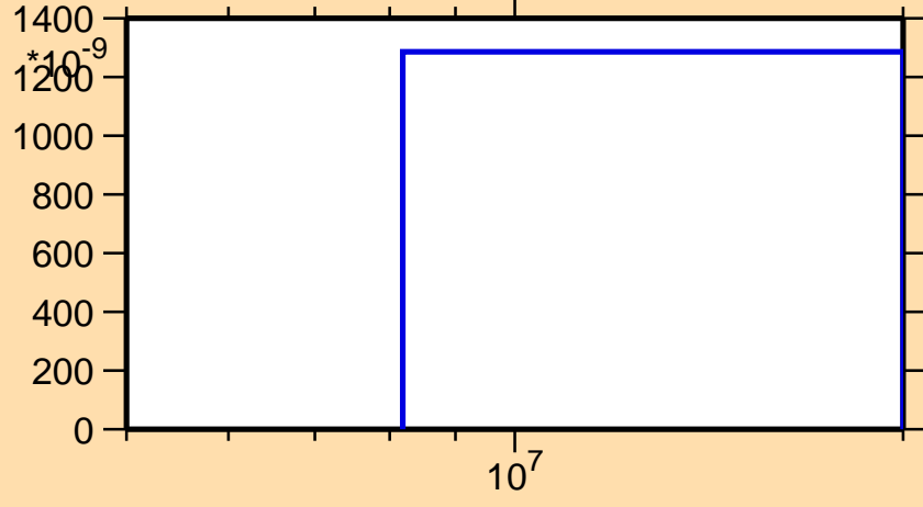
\sigma vs. E for ^{250}\text{Md}(n,nd)
