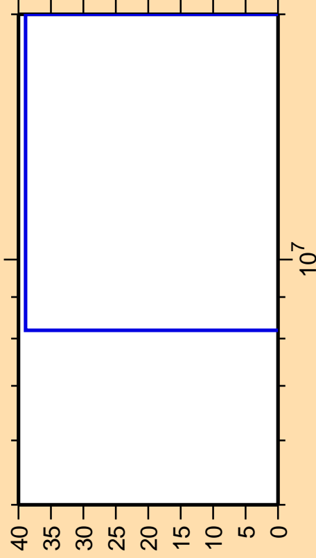
\Delta\sigma/\sigma vs. E for ^{250}\text{Md}(n,nd)
