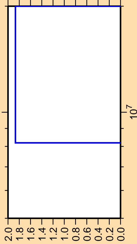
\Delta\sigma/\sigma vs. E for ^{250}\text{Md} (mt 34)
