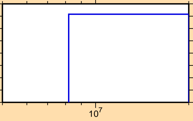
\sigma vs. E for ^{250}\text{Md}(n,\text{He3})
