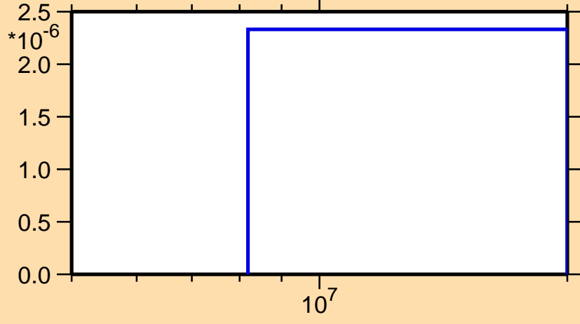
\sigma vs. E for ^{250}\text{Md}(n,2np)
