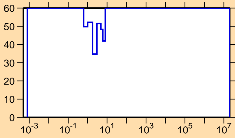
\Delta\sigma/\sigma vs. E for ^{250}\text{Md}(n,\gamma)
