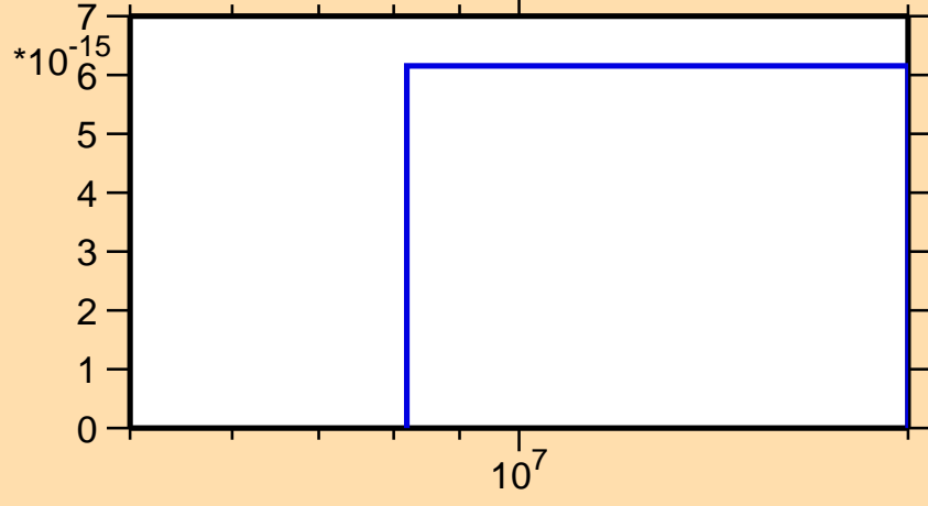
\sigma vs. E for ^{250}\text{Md}(n,\text{pt})
