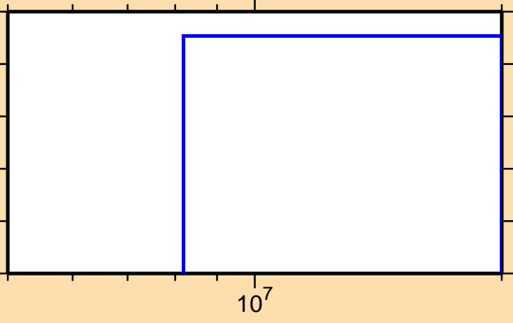
\sigma vs. E for ^{250}\text{Md}(\text{mt } 11)
