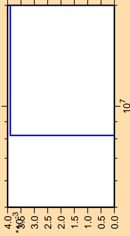
\Delta\sigma/\sigma vs. E for ^{250}\text{Md}(\text{mt } 11)
