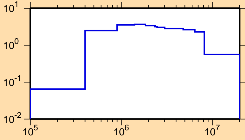
\sigma vs. E for ^{250}\text{Md}(n,\text{inel.})
