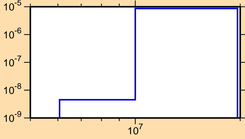
\sigma vs. E for ^{251}\text{Md} (mt 45)
