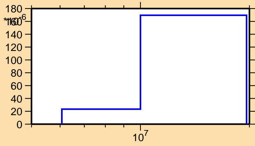
\sigma vs. E for ^{251}\text{Md}(n,2n\alpha)
