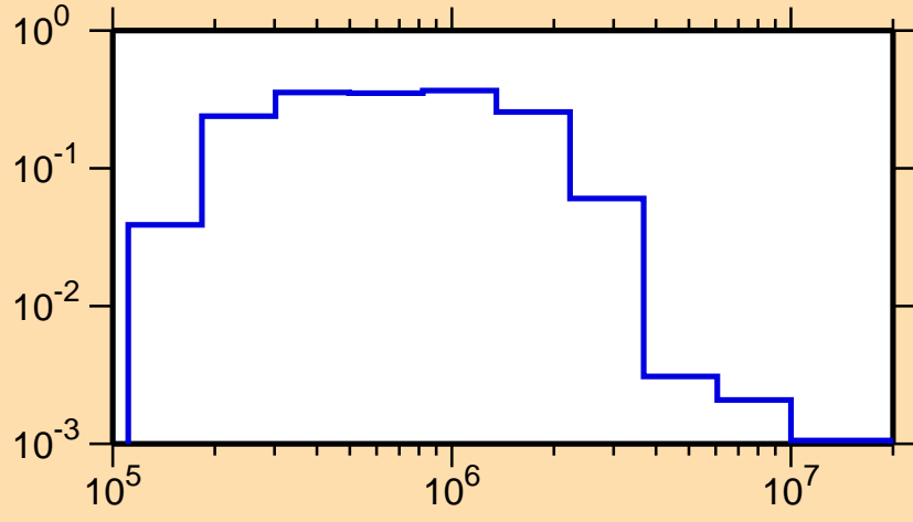
\sigma vs. E for ^{251}\text{Md}(n,n_3)
