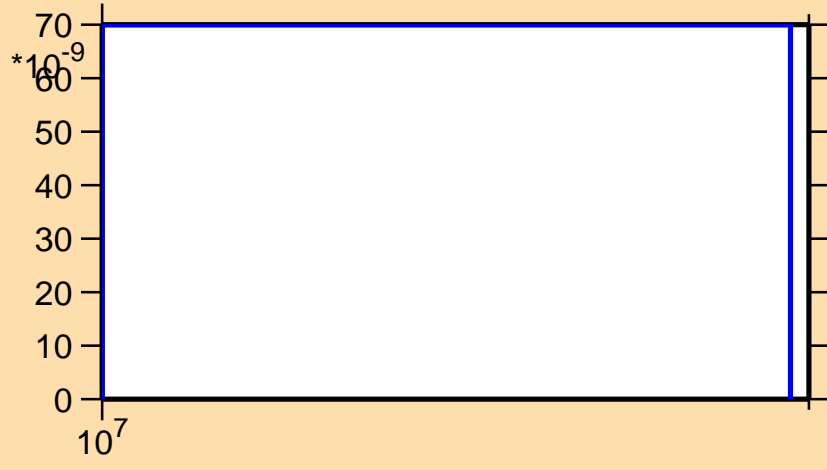
\sigma vs. E for ^{251}\text{Md}(n,nt)
