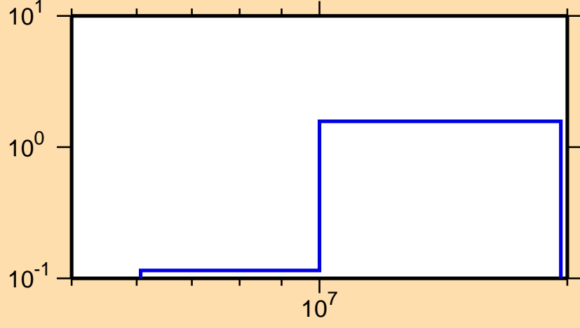
\sigma vs. E for ^{251}\text{Md}(n,2n)
