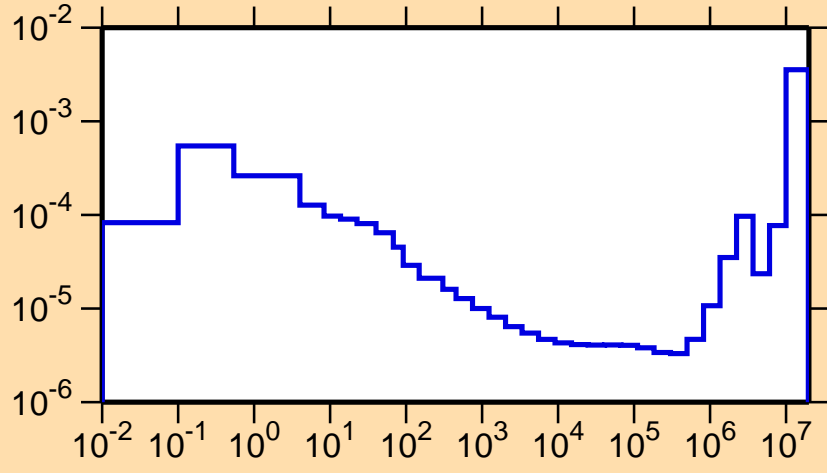
\sigma vs. E for ^{251}\text{Md}(n,\alpha)
