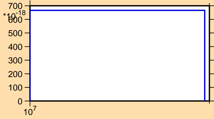
\sigma vs. E for ^{251}\text{Md}(\text{mt } 42)
