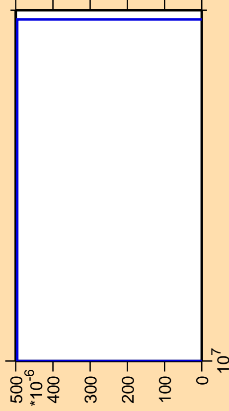
\Delta\sigma/\sigma vs. E for ^{251}\text{Md}(\text{mt } 42)
