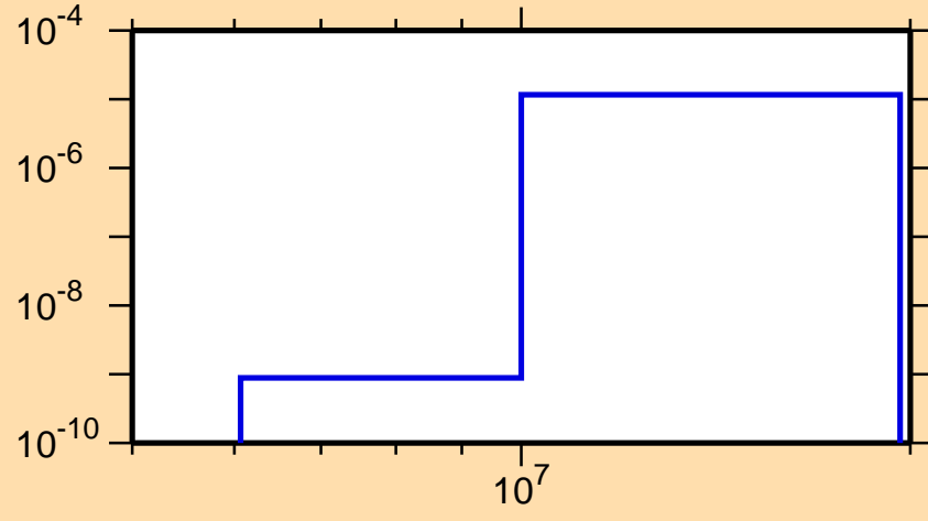
\sigma vs. E for ^{251}\text{Md}(\text{mt117})
