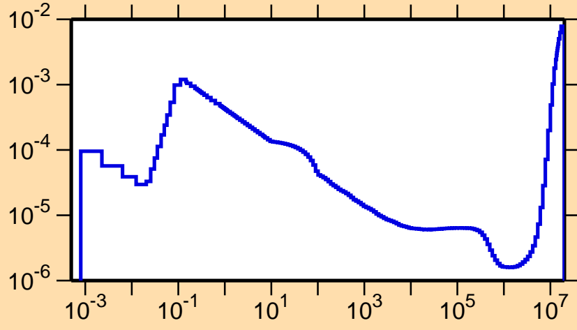
\sigma vs. E for ^{252}\text{Md}(n,\alpha)
