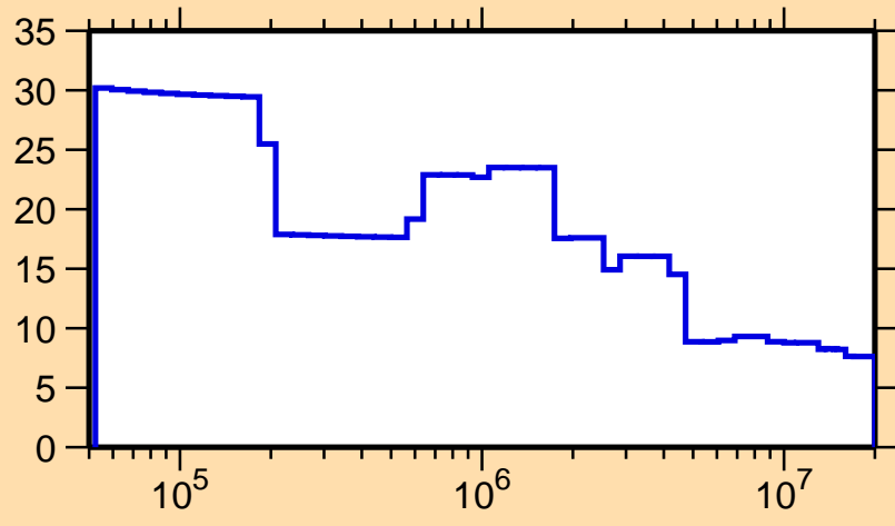
\Delta\sigma/\sigma vs. E for ^{252}\text{Md}(n,\text{nonel.})
