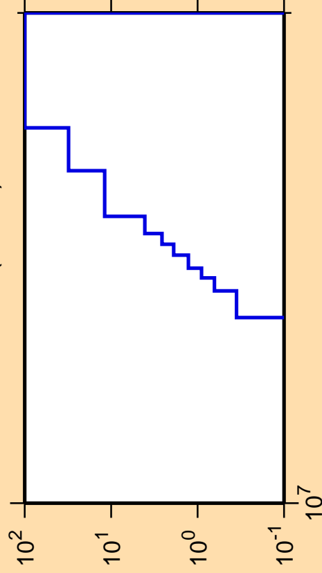
\Delta\sigma/\sigma vs. E for ^{252}\text{Md} (mt 45)
