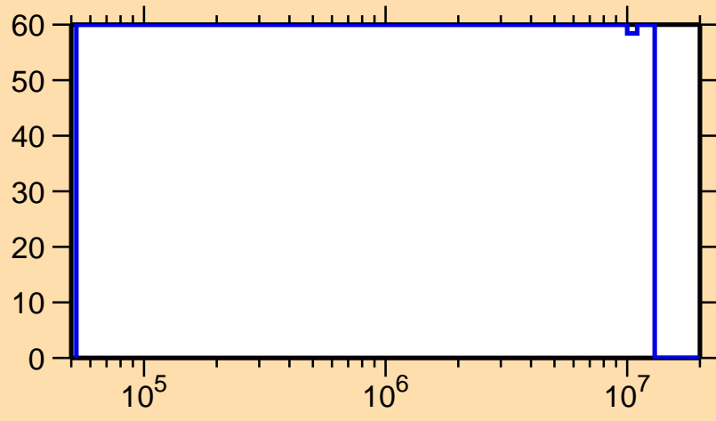
\Delta\sigma/\sigma vs. E for ^{252}\text{Md}(n,n_1)
