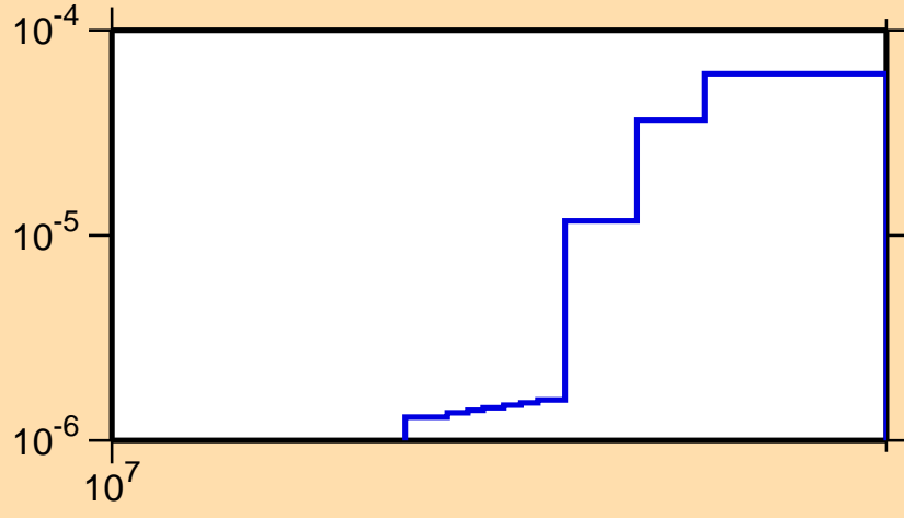
\sigma vs. E for ^{252}\text{Md}(n,3n\alpha)
