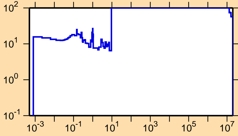
\Delta\sigma/\sigma vs. E for ^{252}\text{Md}(n,f)
