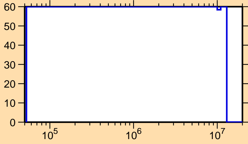
\Delta\sigma/\sigma vs. E for ^{252}\text{Md}(n,n_1)
