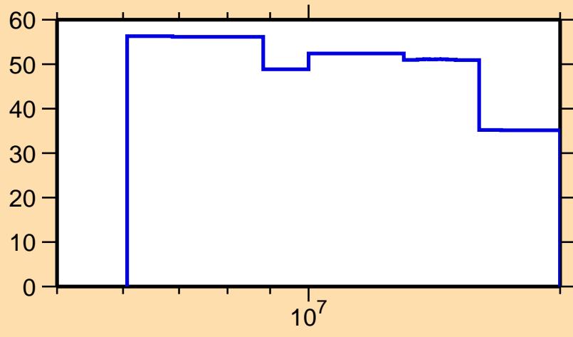
\Delta\sigma/\sigma vs. E for ^{252}\text{Md}(n,2n)
