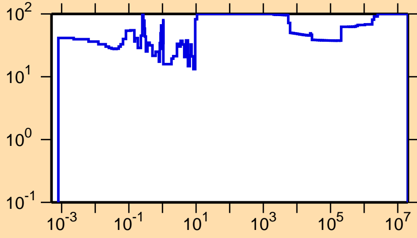
\Delta\sigma/\sigma vs. E for ^{252}\text{Md}(n,\gamma)
