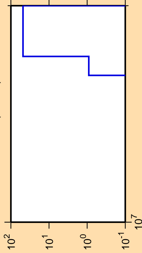
\Delta\sigma/\sigma vs. E for ^{252}\text{Md} (mt 34)
