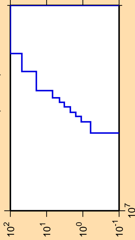
\Delta\sigma/\sigma vs. E for ^{252}\text{Md}(\text{mt117})
