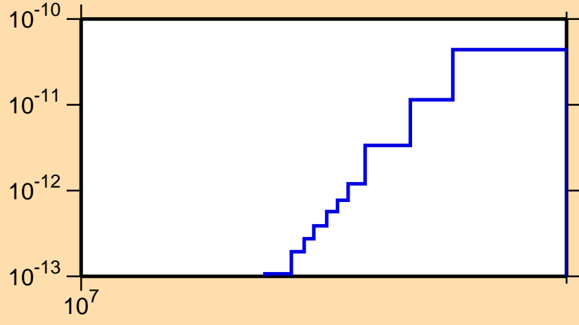
\sigma vs. E for ^{252}\text{Md}(\text{mt117})
