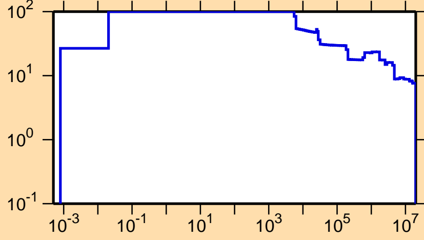
\Delta\sigma/\sigma vs. E for ^{252}\text{Md}(n,\text{nonel.})
