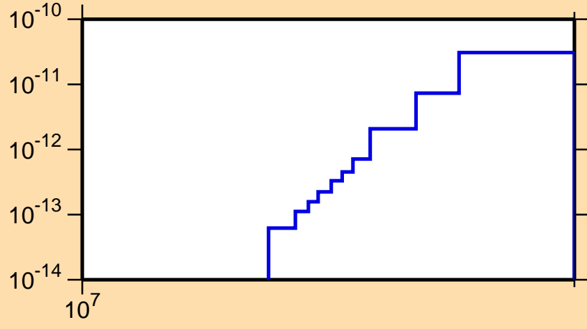
\sigma vs. E for ^{252}\text{Md} (mt 45)
