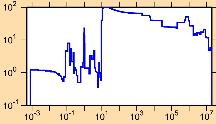
\Delta\sigma/\sigma vs. E for ^{252}\text{Md}(n,\text{el.})
