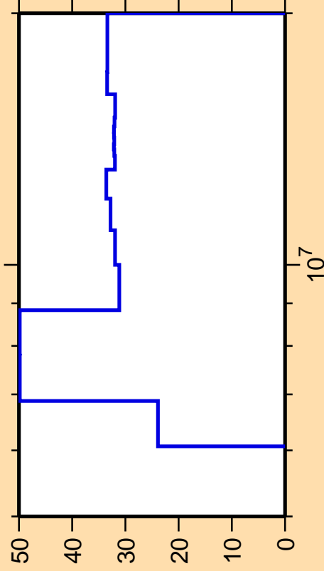
\Delta\sigma/\sigma vs. E for ^{252}\text{Md}(n,n\text{cont.})
