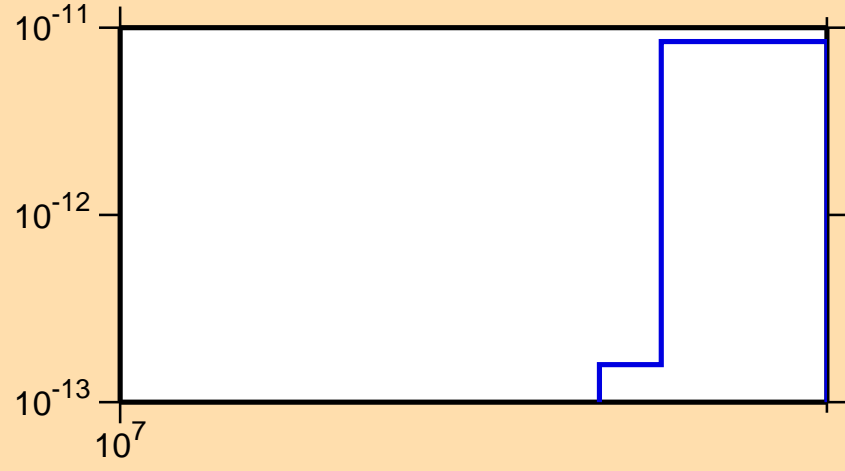
\sigma vs. E for ^{252}\text{Md} (mt 34)
