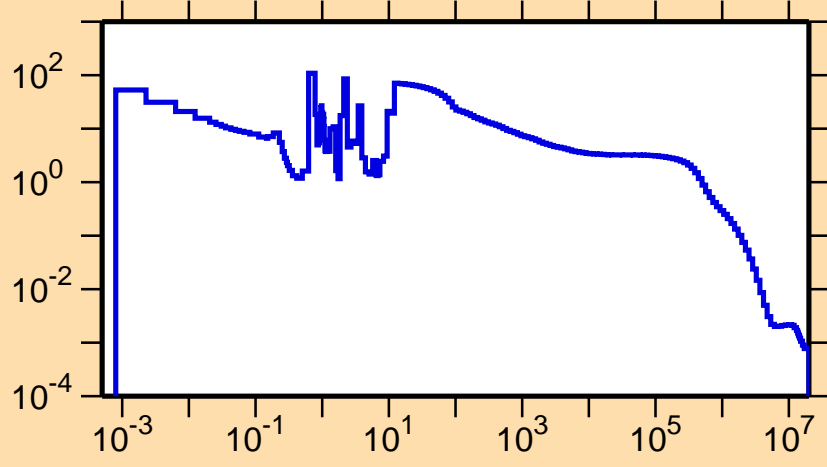
\sigma vs. E for ^{252}\text{Md}(n,\gamma)
