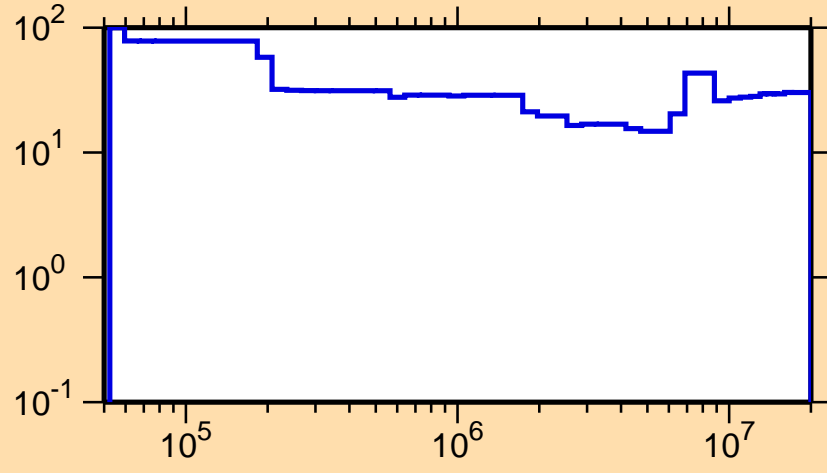
\Delta\sigma/\sigma vs. E for ^{252}\text{Md}(n,\text{inel.})
