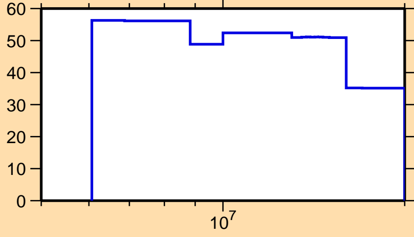
\Delta\sigma/\sigma vs. E for ^{252}\text{Md}(n,2n)
