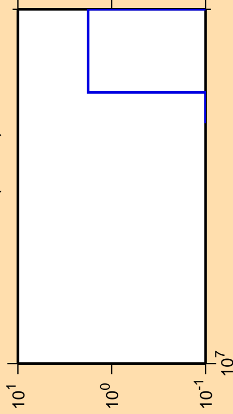
\Delta\sigma/\sigma vs. E for ^{252}\text{Md} (mt 11)
