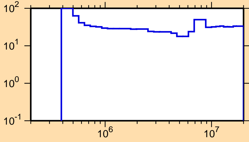
\Delta\sigma/\sigma vs. E for ^{252}\text{Md}(n,n\text{cont.})
