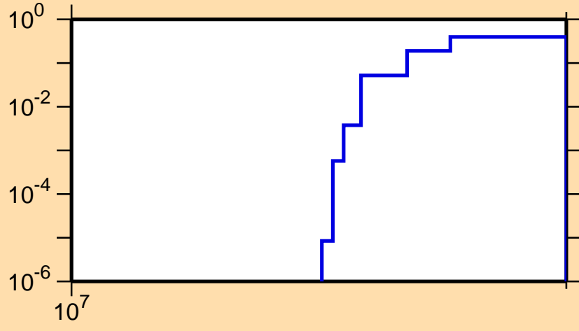
\sigma vs. E for ^{252}\text{Md}(n,3n)
