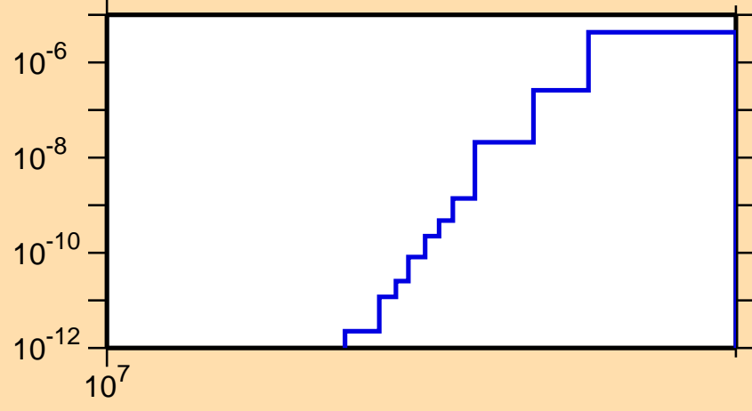
\sigma vs. E for ^{252}\text{Md}(n,nt)
