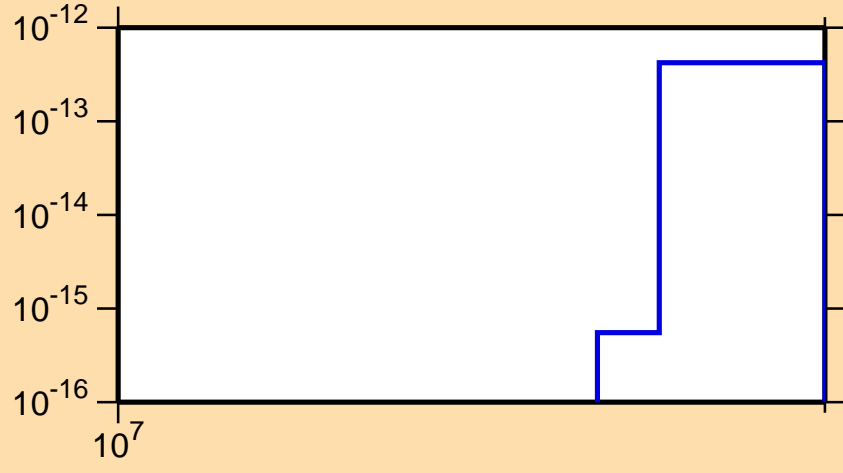
\sigma vs. E for ^{252}\text{Md} (mt 11)
