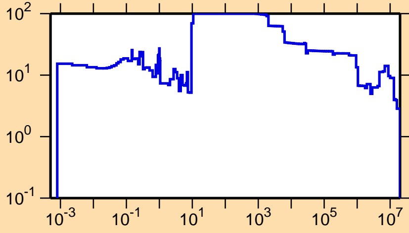
\Delta\sigma/\sigma vs. E for ^{252}\text{Md}(n,\text{tot.})
