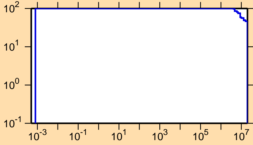
\Delta\sigma/\sigma vs. E for ^{252}\text{Md}(n,p)
