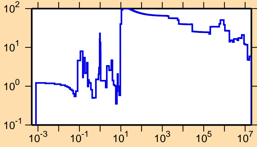
\Delta\sigma/\sigma vs. E for ^{252}\text{Md}(n,el.)
