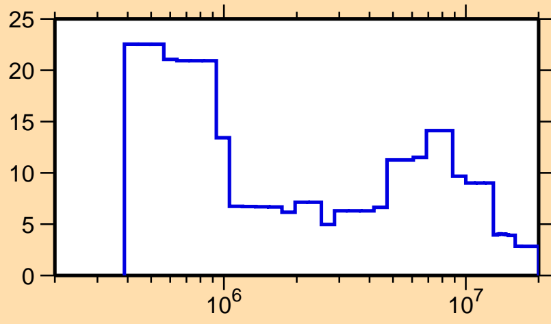
\Delta\sigma/\sigma vs. E for ^{252}\text{Md}(n,\text{tot.})
