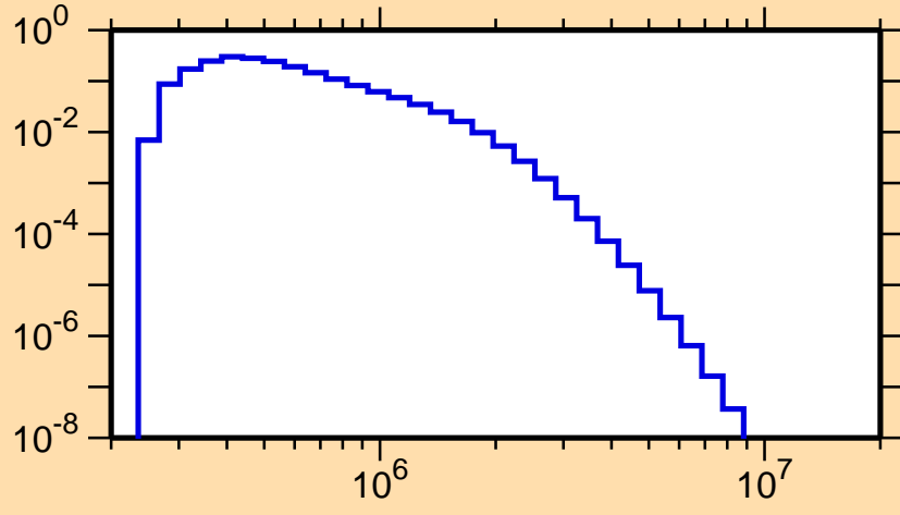
\sigma vs. E for ^{252}\text{Md}(n,n_4)
