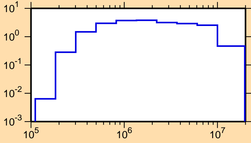
\sigma vs. E for ^{252}\text{Md}(n,\text{inel.})
