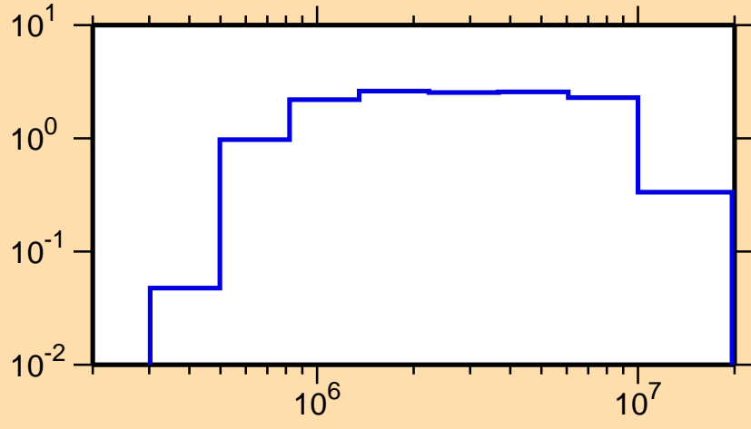
\sigma vs. E for ^{252}\text{Md}(n,n\text{cont.})
