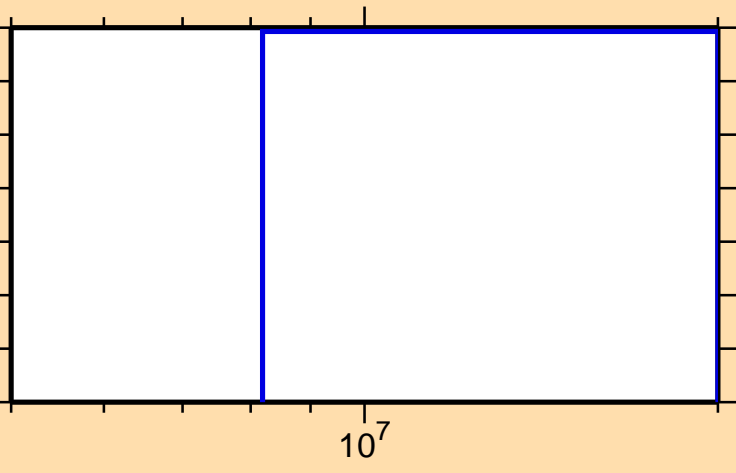
\sigma vs. E for ^{252}\text{Md}(n,p\alpha)
