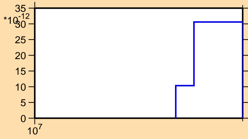
\sigma vs. E for ^{253}\text{Md}(\text{mt117})
