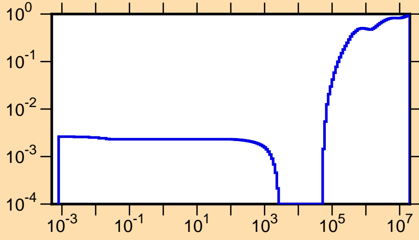
\mu vs. E for ^{254}\text{Md}(\text{mt251})
