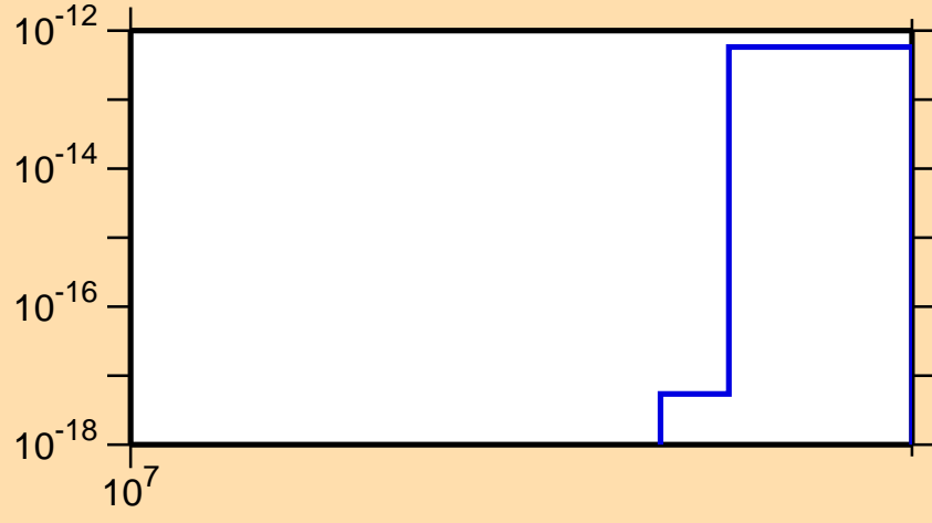
\sigma vs. E for ^{254}\text{Md} (mt 42)
