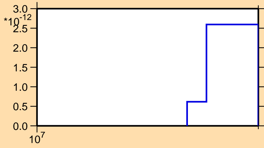
\sigma vs. E for ^{254}\text{Md} (mt 45)
