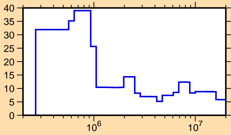
\Delta\sigma/\sigma vs. E for ^{254}\text{Md}(n, el.)
