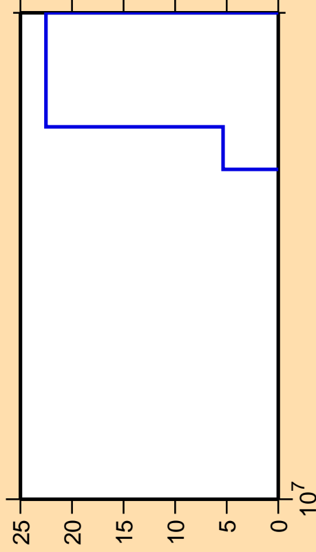
\Delta\sigma/\sigma vs. E for ^{254}\text{Md} (mt 45)
