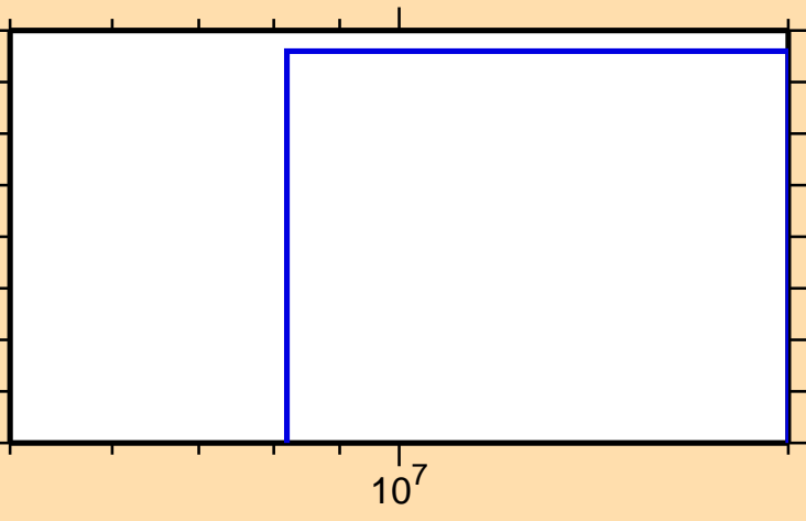
\sigma vs. E for ^{254}\text{Md} (mt 34)
