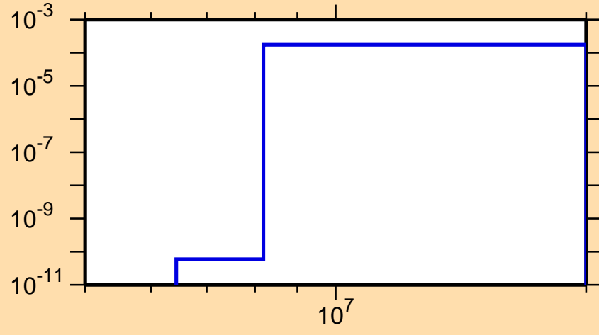
\sigma vs. E for ^{254}\text{Md}(n,t)
