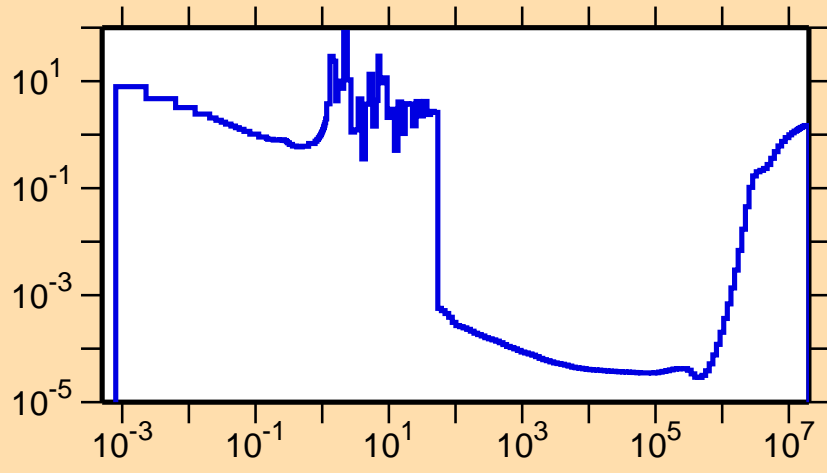
\sigma vs. E for ^{255}\text{Md}(n,f)
