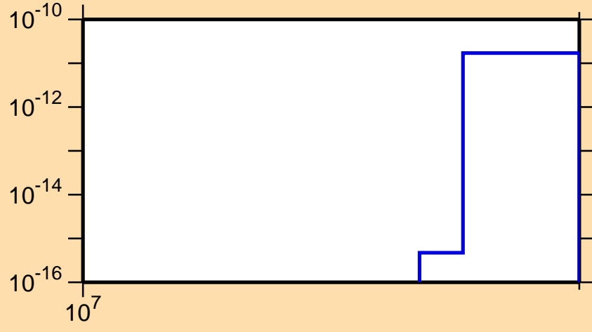
\sigma vs. E for ^{255}\text{Md} (mt 11)
