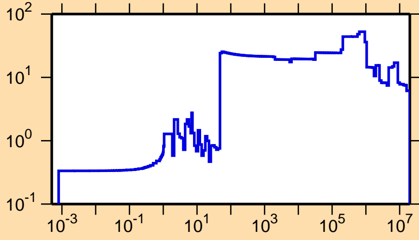
\Delta\sigma/\sigma vs. E for ^{255}\text{Md}(n,el.)
