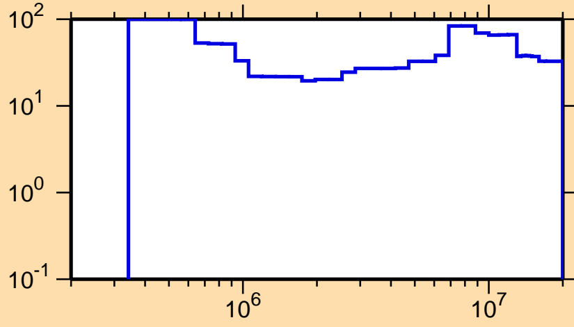
\Delta\sigma/\sigma vs. E for ^{255}\text{Md}(n,n\text{cont.})
