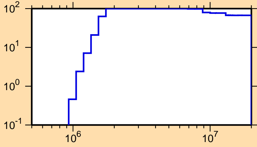
\Delta\sigma/\sigma vs. E for ^{255}\text{Md}(n,p)
