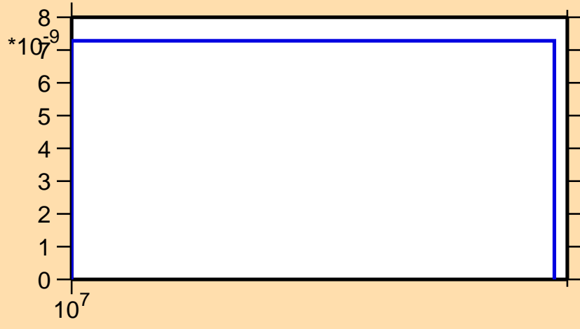
\sigma vs. E for ^{255}\text{Md}(n,3n\alpha)
