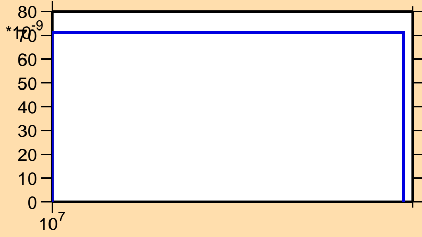
\sigma vs. E for ^{255}\text{Md}(n,2np)
