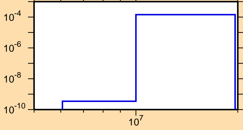
\sigma vs. E for ^{255}\text{Md}(n,t)
