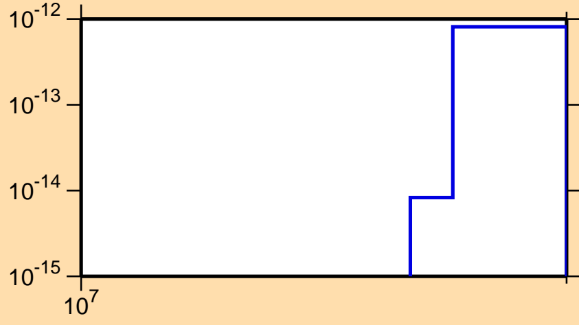
\sigma vs. E for ^{256}\text{Md} (mt 34)
