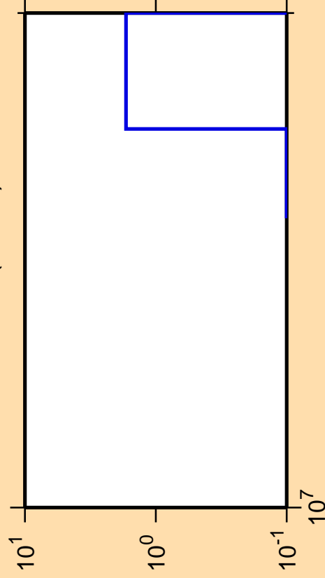
\Delta\sigma/\sigma vs. E for ^{256}\text{Md} (mt 42)
