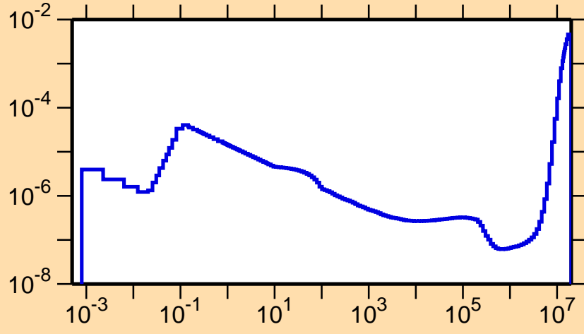
\sigma vs. E for ^{256}\text{Md}(n,\alpha)
