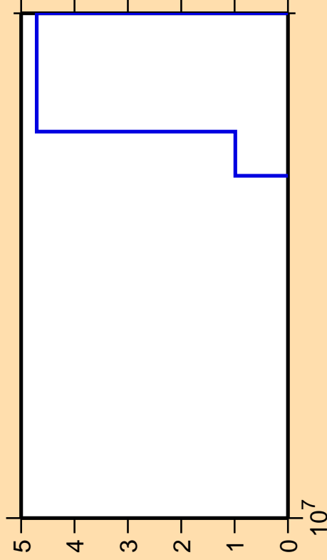
\Delta\sigma/\sigma vs. E for ^{256}\text{Md}(\text{mt } 45)
