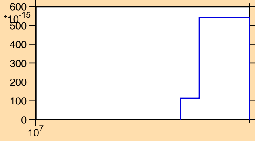
\sigma vs. E for ^{256}\text{Md}(\text{mt } 45)
