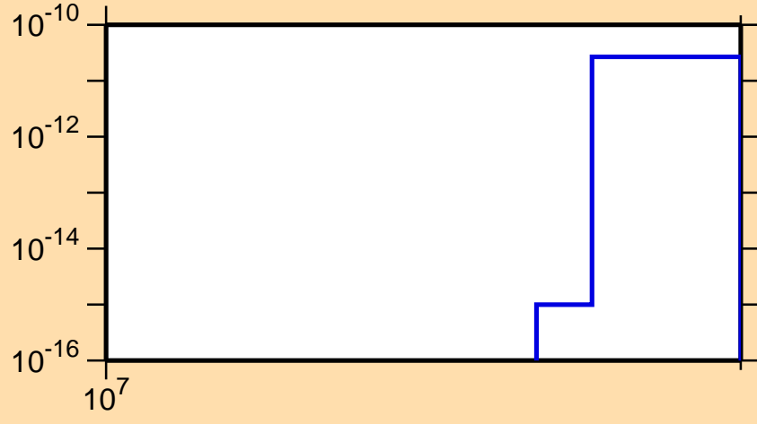
\sigma vs. E for ^{256}\text{Md} (mt 11)
