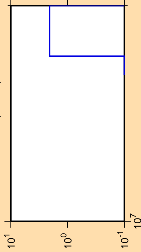
\Delta\sigma/\sigma vs. E for ^{256}\text{Md} (mt 34)
