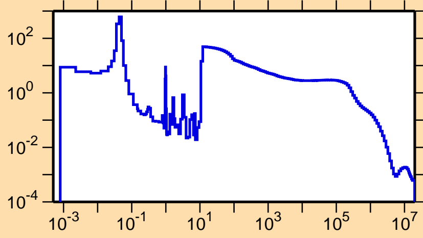
\sigma vs. E for ^{256}\text{Md}(n,\gamma)
