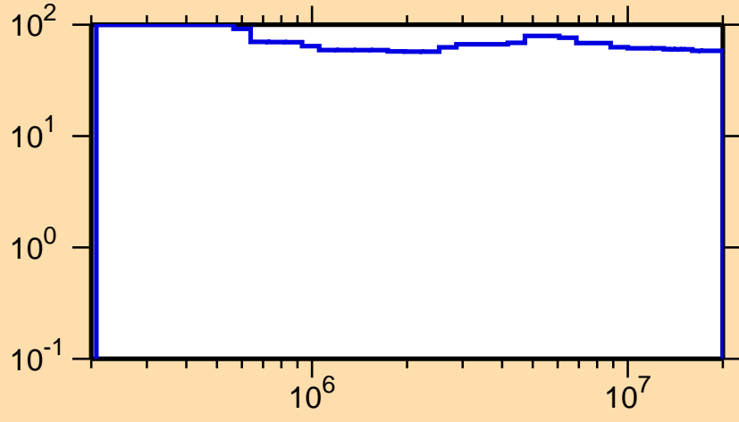
\Delta\sigma/\sigma vs. E for ^{256}\text{Md}(n,n\text{cont.})
