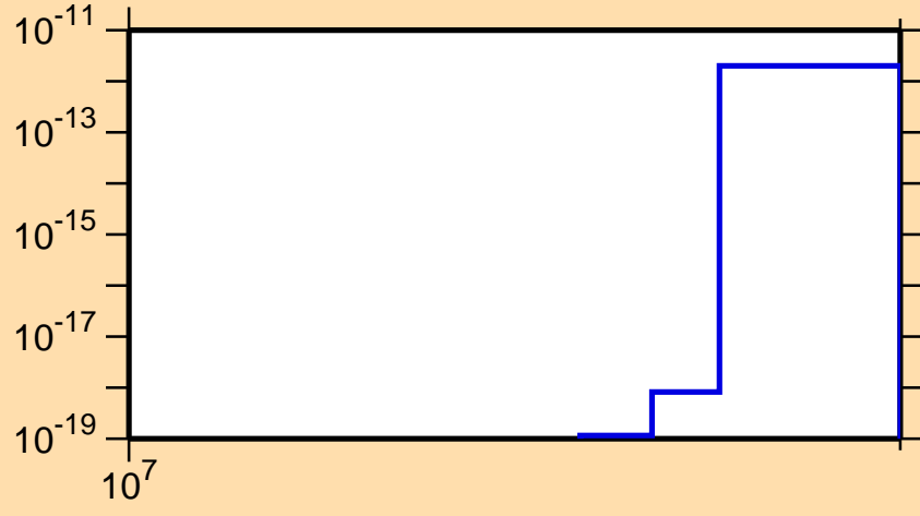
\sigma vs. E for ^{256}\text{Md} (mt 42)
