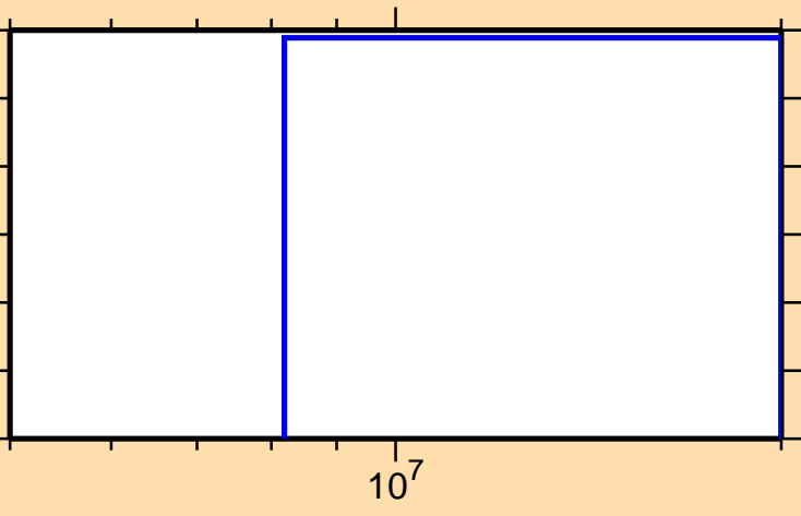
\sigma vs. E for ^{256}\text{Md}(n,nd)
