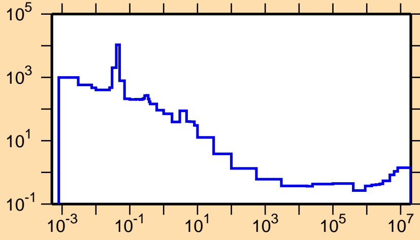
\sigma vs. E for ^{256}\text{Md}(n,f)
