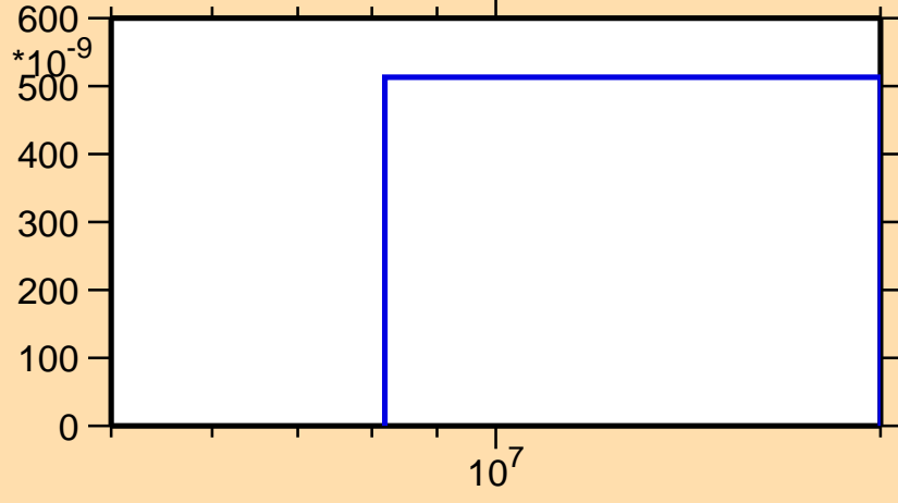
\sigma vs. E for ^{256}\text{Md}(n,nt)
