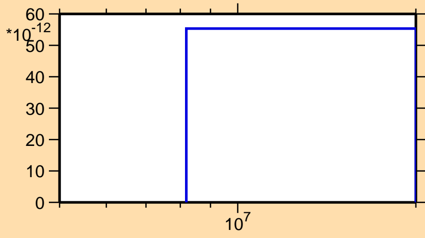
\sigma vs. E for ^{256}\text{Md}(n,\text{He3})
