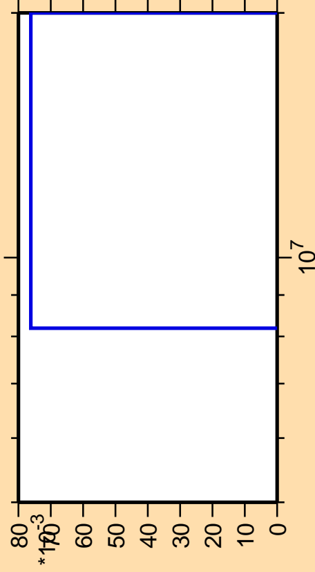
\Delta\sigma/\sigma vs. E for ^{256}\text{Md}(\text{mt } 45)
