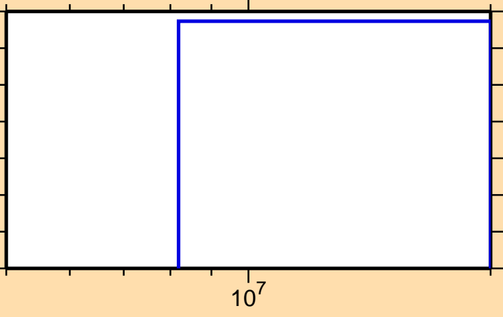
\sigma vs. E for ^{256}\text{Md}(\text{mt } 45)
