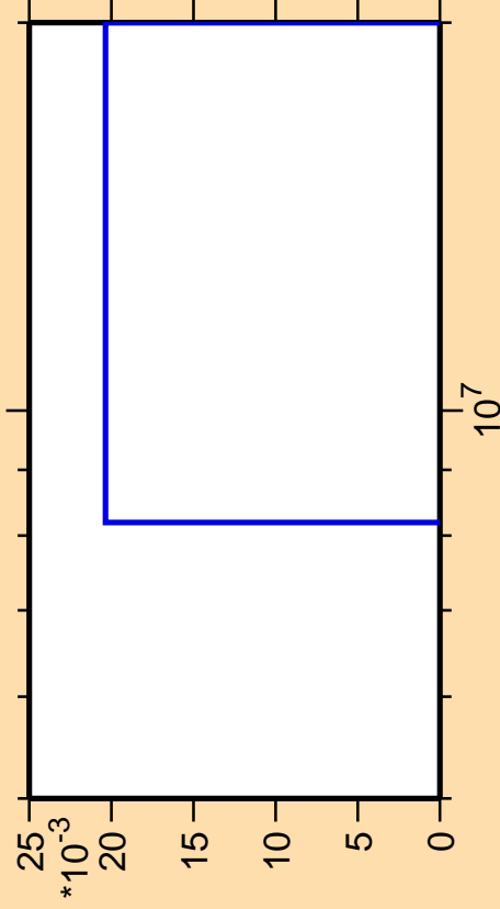
\Delta\sigma/\sigma vs. E for ^{258}\text{Md}(\text{mt } 42)
