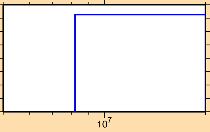
\sigma vs. E for ^{258}\text{Md}(n,2np)
