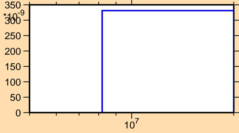
\sigma vs. E for ^{258}\text{Md}(n,\text{nd})
