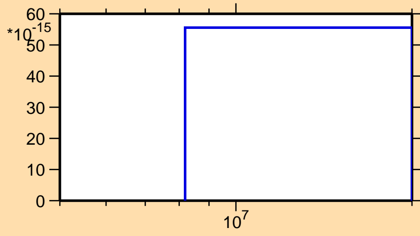
\sigma vs. E for ^{258}\text{Md}(\text{mt } 11)
