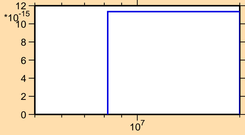
\sigma vs. E for ^{258}\text{Md}(\text{mt } 42)
