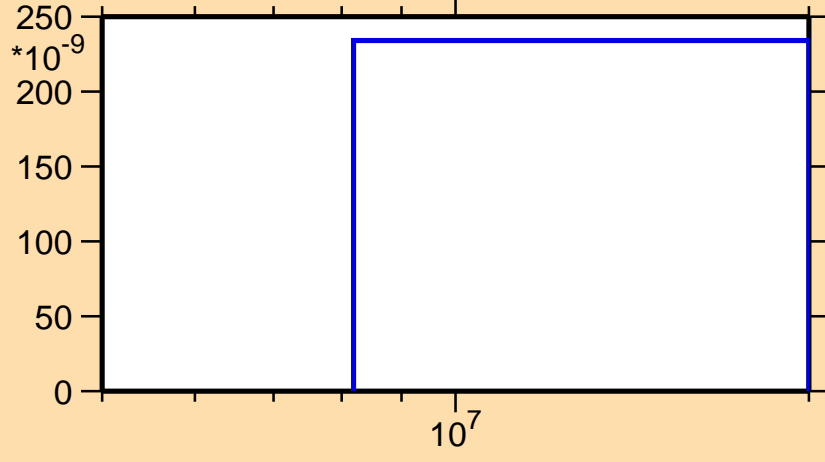
\sigma vs. E for ^{258}\text{Md}(n,nt)
