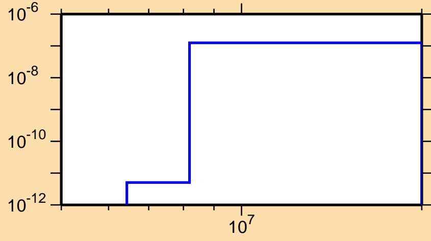
\sigma vs. E for ^{258}\text{Md}(n,2n\alpha)
