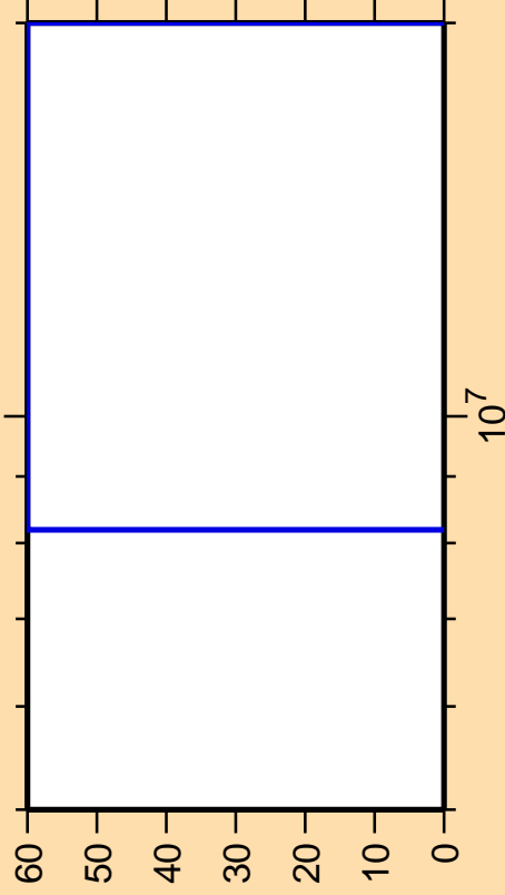
\Delta\sigma/\sigma vs. E for ^{258}\text{Md}(n,2np)
