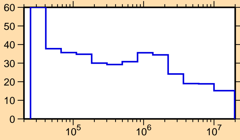
\Delta\sigma/\sigma vs. E for ^{258}\text{Md}(n,n\text{onel.})
