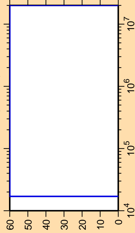
\Delta\sigma/\sigma vs. E for ^{258}\text{Md}(n,\text{inel.})
