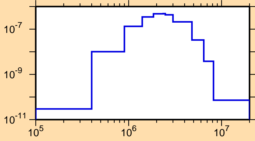
\sigma vs. E for ^{258}\text{Md}(n,n_3)
