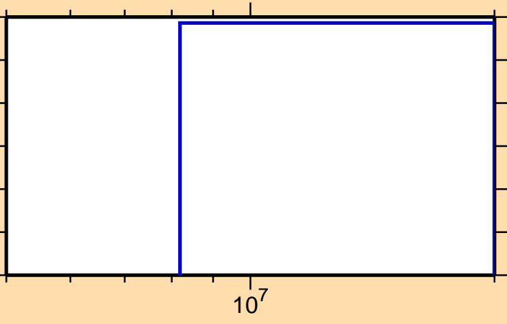
\sigma vs. E for ^{258}\text{Md}(n,nt)
