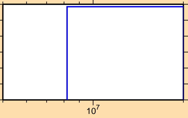
\sigma vs. E for ^{258}\text{Md}(n,nd)
