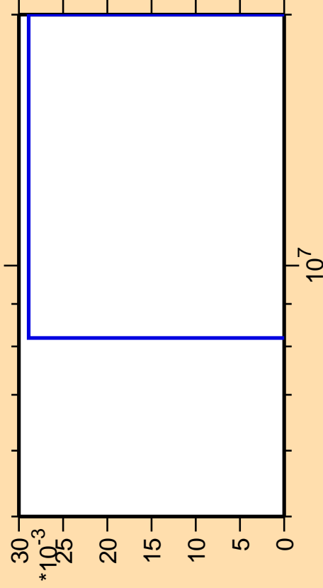
\Delta\sigma/\sigma vs. E for ^{258}\text{Md} (mt 34)
