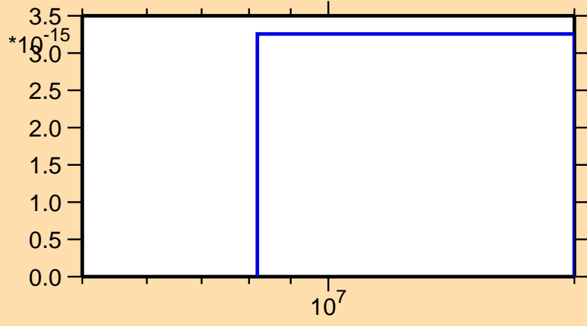
\sigma vs. E for ^{258}\text{Md} (mt 34)
