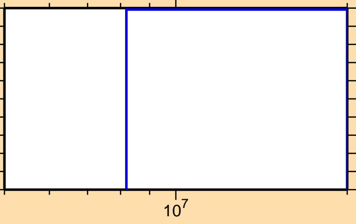
\sigma vs. E for ^{258}\text{Md}(n,3n\alpha)
