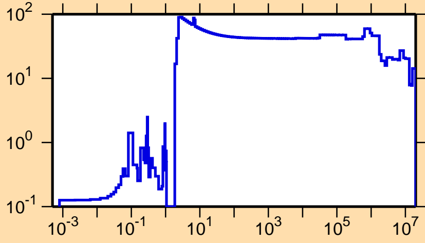
\Delta\sigma/\sigma vs. E for ^{259}\text{Md}(n,el.)
