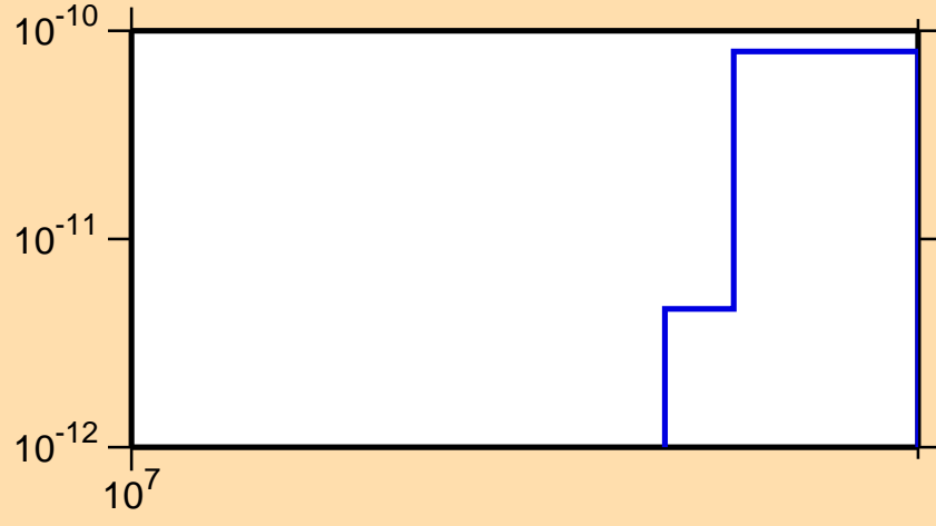
\sigma vs. E for ^{259}\text{Md}(n,\text{He3})
