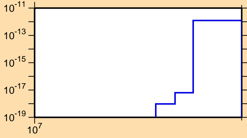
\sigma vs. E for ^{259}\text{Md} (mt 42)
