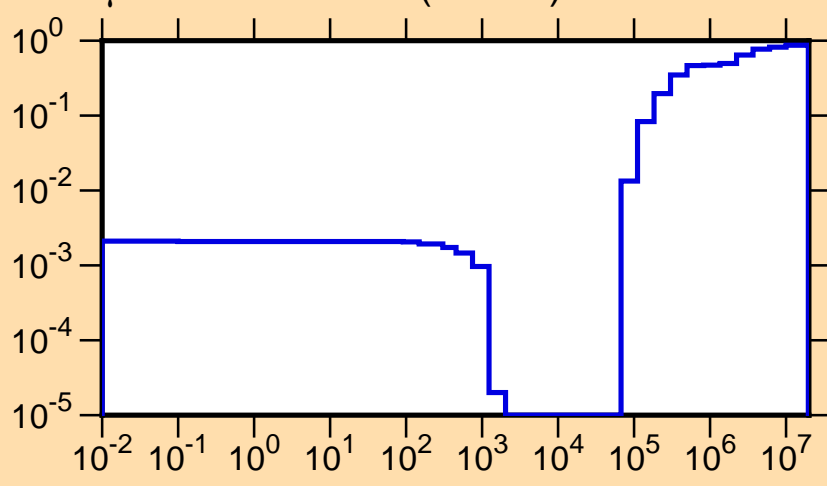
\mu vs. E for ^{259}\text{Md}(\text{mt251})
