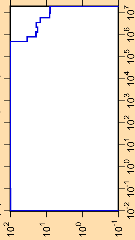
\Delta\mu/\mu vs. E for ^{259}\text{Md}(\text{mt251})
