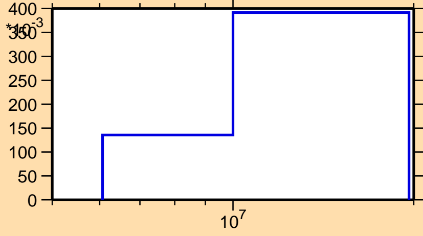
\sigma vs. E for ^{259}\text{Md}(n,2n)
