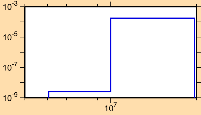
\sigma vs. E for ^{259}\text{Md}(n,d)
