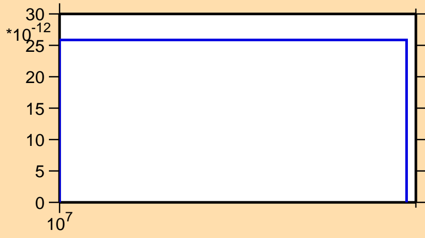
\sigma vs. E for ^{259}\text{Md}(n,3n\alpha)
