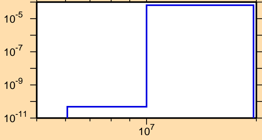
\sigma vs. E for ^{259}\text{Md}(n,t)
