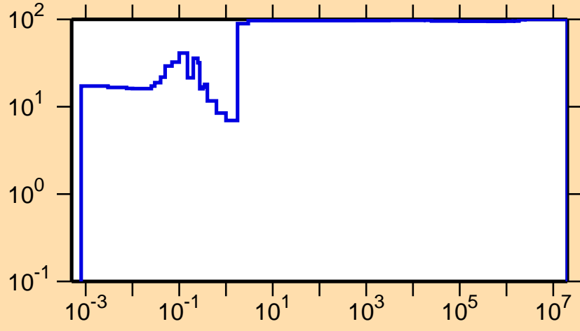
\Delta\sigma/\sigma vs. E for ^{259}\text{Md}(n,\gamma)
