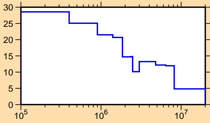
\Delta\sigma/\sigma vs. E for ^{259}\text{Md}(n,\text{tot.})
