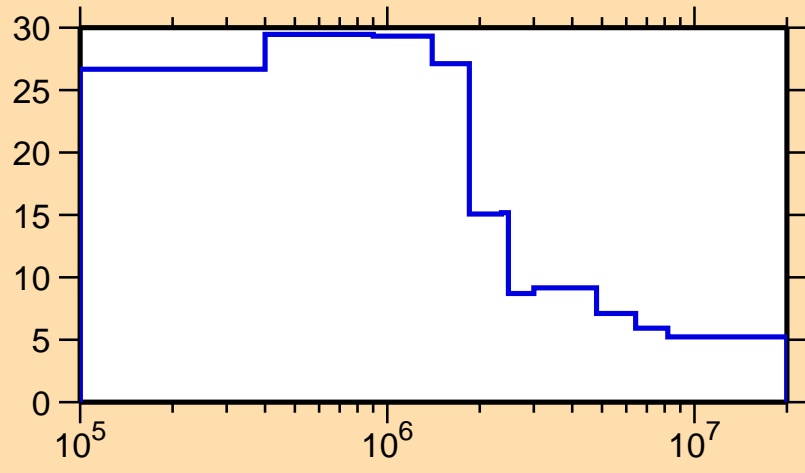
\Delta\sigma/\sigma vs. E for ^{259}\text{Md}(n,\text{nonel.})
