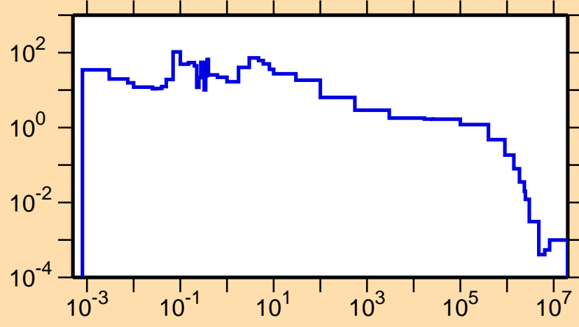
\sigma vs. E for ^{259}\text{Md}(n,\gamma)
