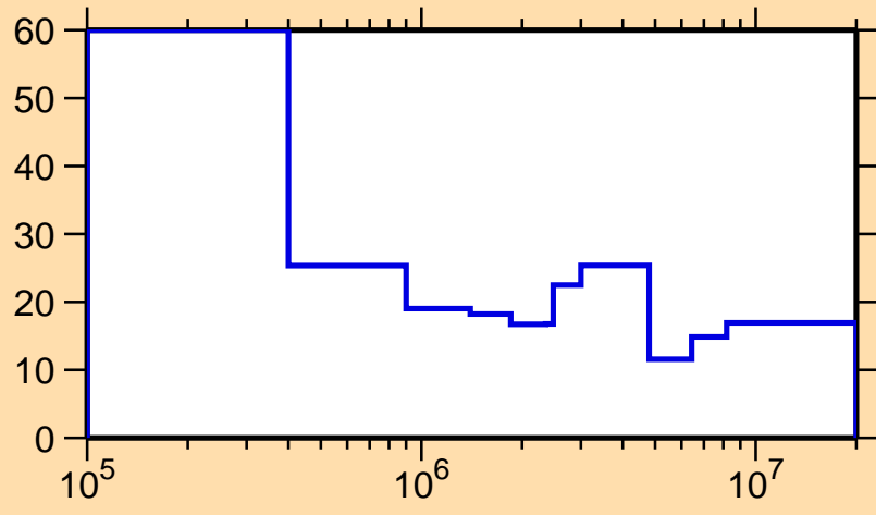
\Delta\sigma/\sigma vs. E for ^{259}\text{Md}(n,f)
