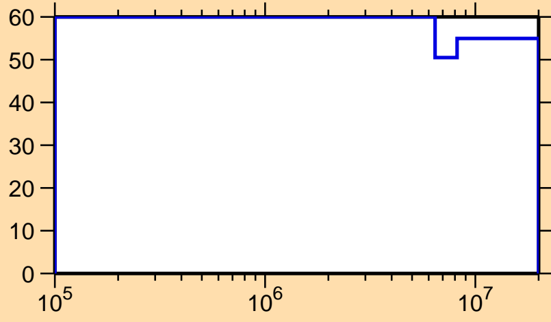
\Delta\sigma/\sigma vs. E for ^{259}\text{Md}(n,\text{inel.})
