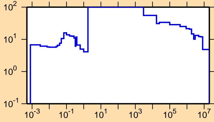
\Delta\sigma/\sigma vs. E for ^{259}\text{Md}(n,\text{tot.})
