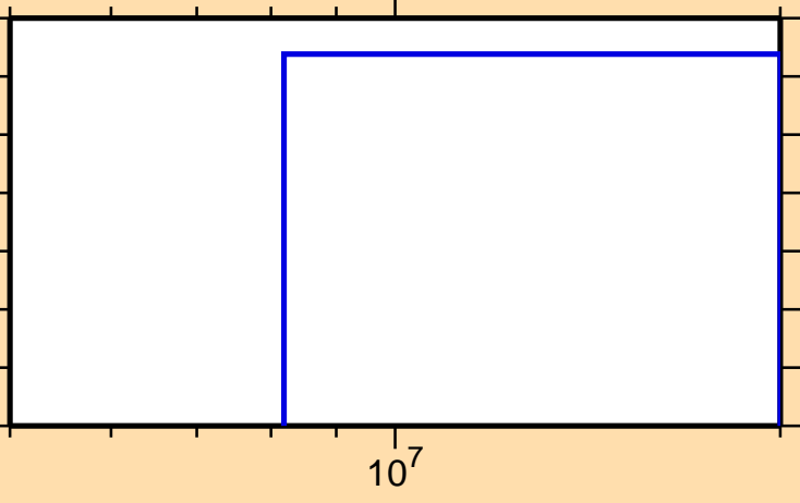
\sigma vs. E for ^{259}\text{Md}(n,\text{nd})
