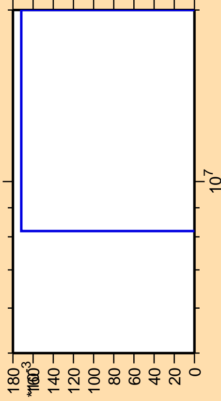
\Delta\sigma/\sigma vs. E for ^{259}\text{Md} (mt 11)
