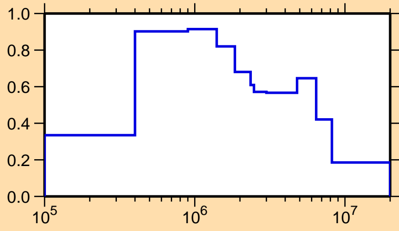
\sigma vs. E for ^{259}\text{Md}(n,\text{inel.})
