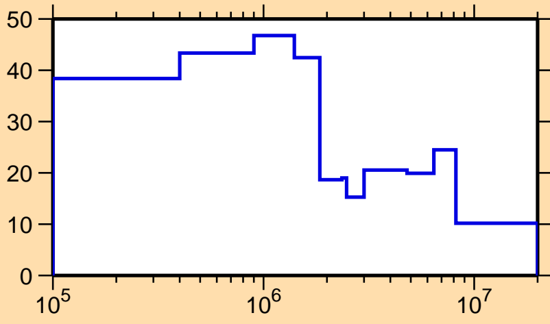
\Delta\sigma/\sigma vs. E for ^{259}\text{Md}(n,\text{el.})
