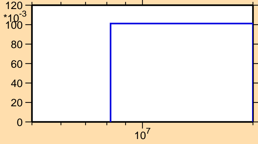
\sigma vs. E for ^{259}\text{Md}(n,3n)
