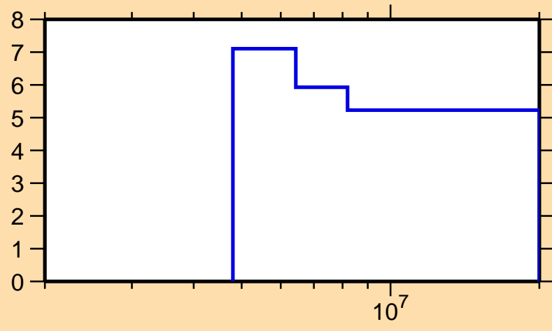
\Delta\sigma/\sigma vs. E for ^{259}\text{Md}(n,\text{nonel.})
