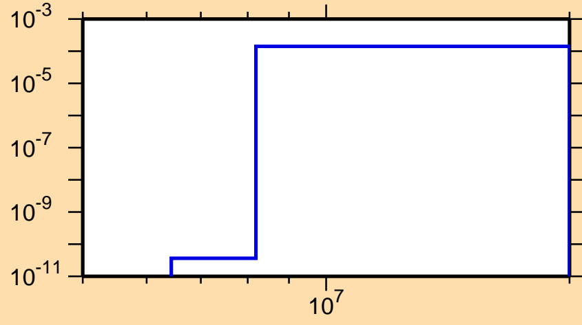
\sigma vs. E for ^{259}\text{Md}(n,d)
