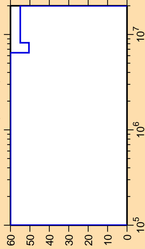
\Delta\sigma/\sigma vs. E for ^{259}\text{Md}(n,\text{inel.})
