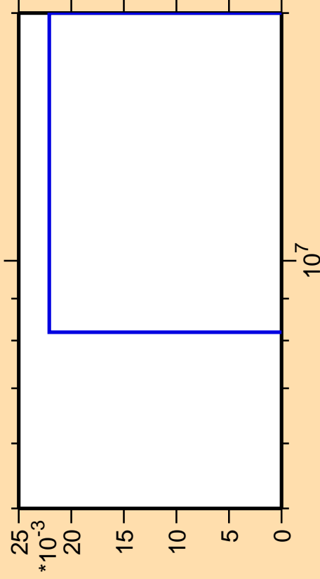
\Delta\sigma/\sigma vs. E for ^{259}\text{Md} (mt 42)
