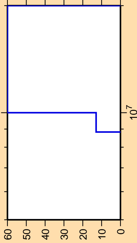
\Delta\sigma/\sigma vs. E for ^{260}\text{Md}(n,2n\alpha)
