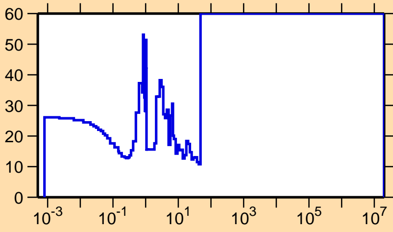
\Delta\sigma/\sigma vs. E for ^{260}\text{Md}(n,\gamma)
