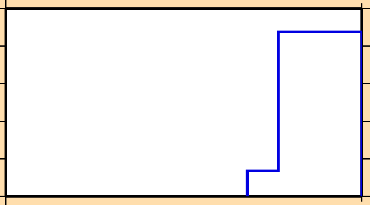
\sigma vs. E for ^{260}\text{Md}(\text{mt } 11)
