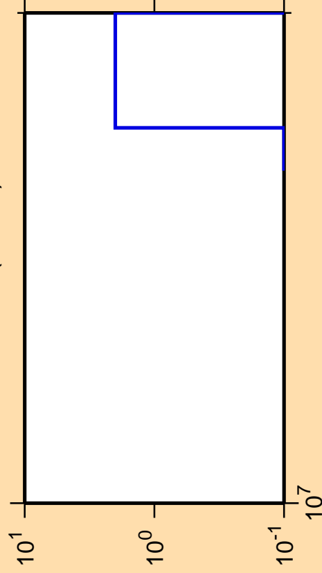
\Delta\sigma/\sigma vs. E for ^{260}\text{Md}(\text{mt } 11)
