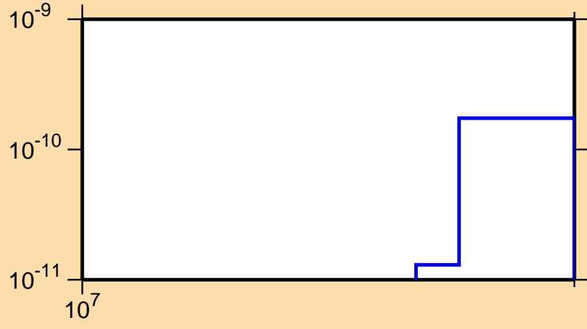
\sigma vs. E for ^{260}\text{Md}(n,\text{He3})
