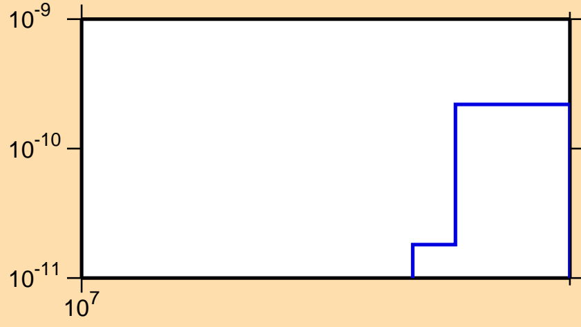
\sigma vs. E for ^{260}\text{Md}(n,3n\alpha)
