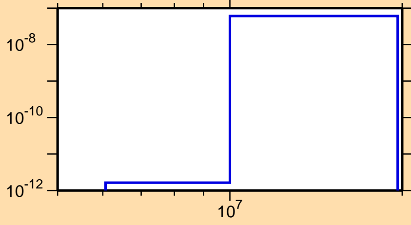
\sigma vs. E for ^{260}\text{Md}(n,2n\alpha)
