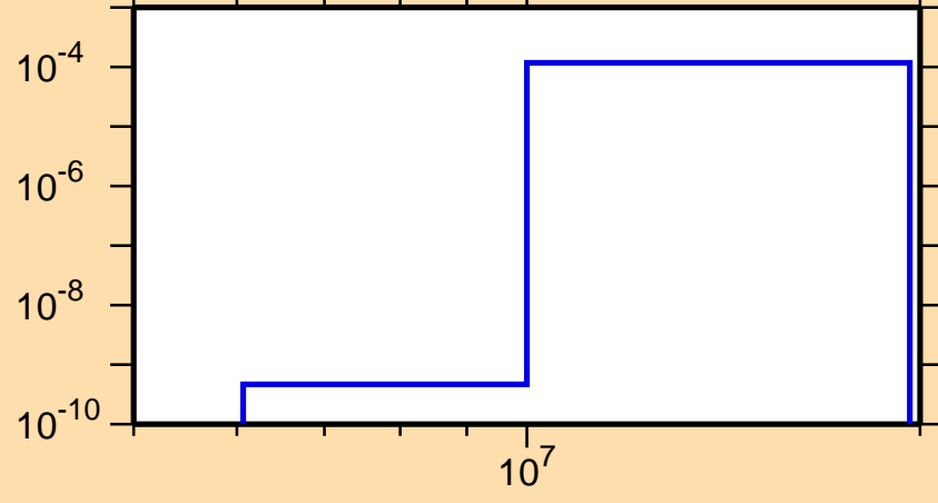
\sigma vs. E for ^{260}\text{Md}(n,d)
