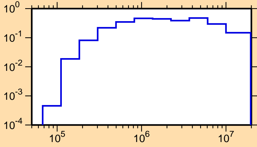
\sigma vs. E for ^{260}\text{Md}(n,n\text{cont.})
