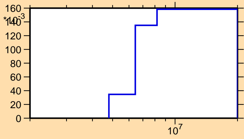
\sigma vs. E for ^{260}\text{Md}(n,2n)
