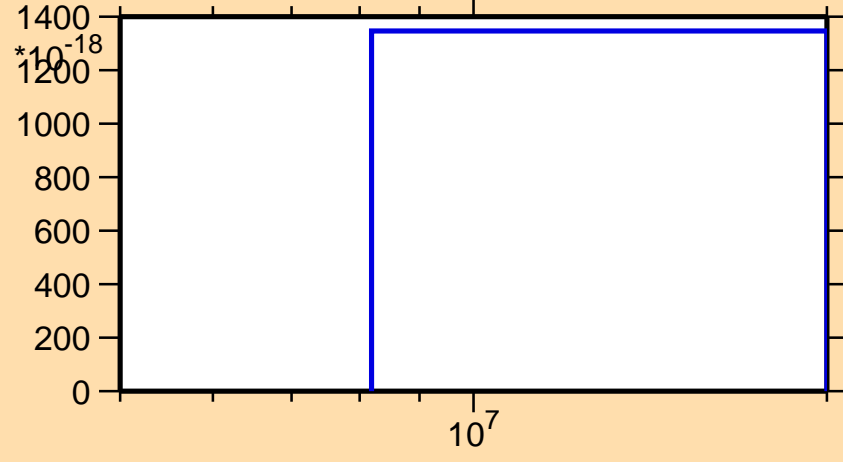
\sigma vs. E for ^{260}\text{Md}(\text{mt } 42)
