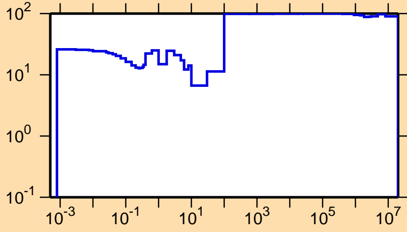
\Delta\sigma/\sigma vs. E for ^{260}\text{Md}(n,\gamma)
