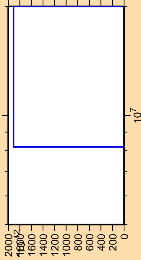
\Delta\sigma/\sigma vs. E for ^{260}\text{Md}(\text{mt } 42)
