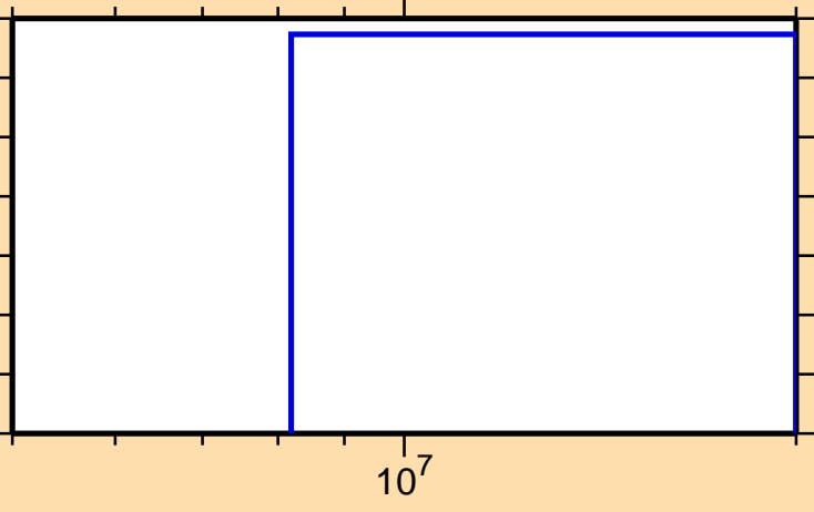
\sigma vs. E for ^{260}\text{Md}(\text{mt } 42)
