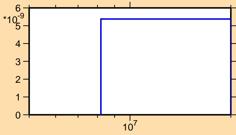
\sigma vs. E for ^{260}\text{Md}(n,2np)
