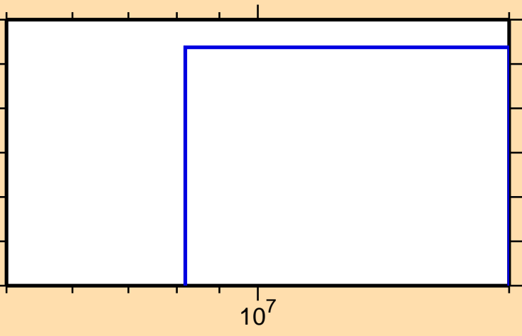
\sigma vs. E for ^{260}\text{Md}(n,3n)
