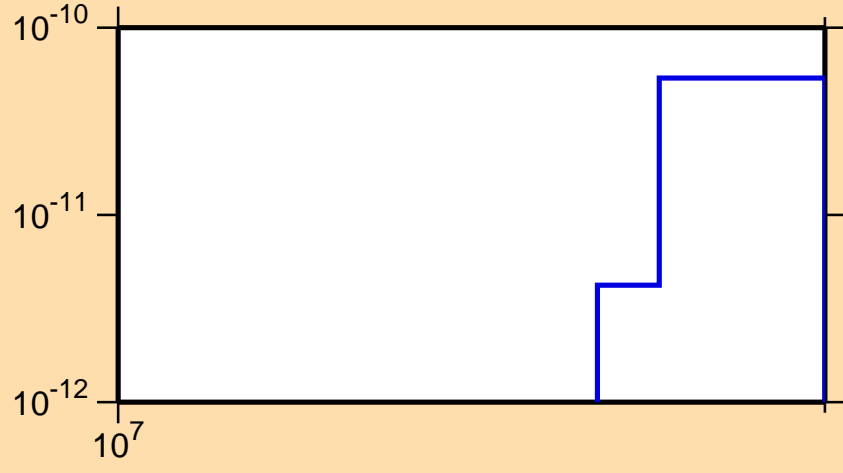
\sigma vs. E for ^{261}\text{Md}(n,3n\alpha)
