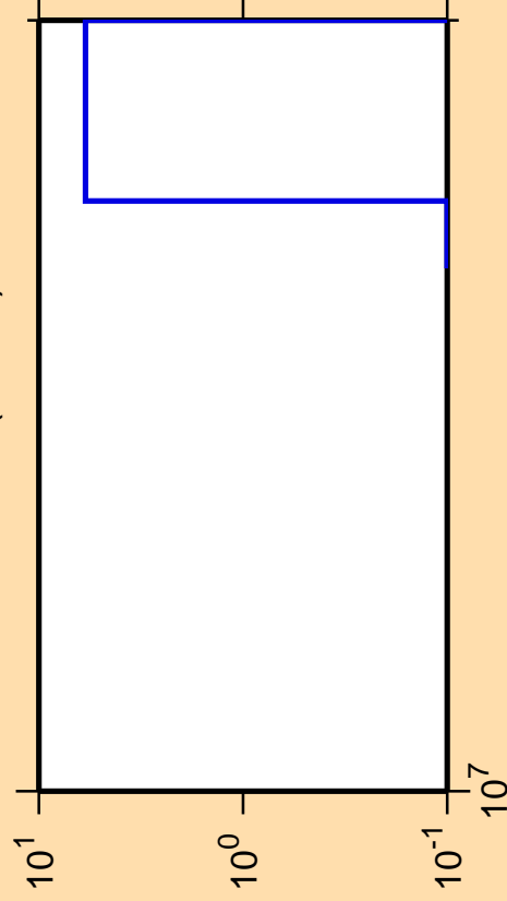
\Delta\sigma/\sigma vs. E for ^{261}\text{Md} (mt 11)
