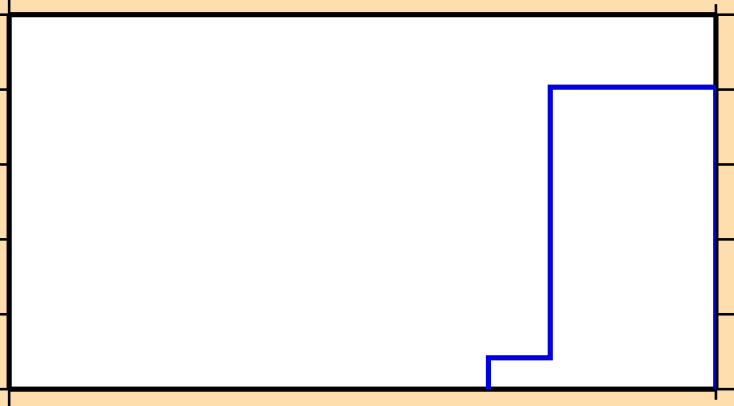
\sigma vs. E for ^{261}\text{Md} (mt 11)
