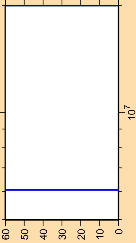
\Delta\sigma/\sigma vs. E for ^{261}\text{Md}(n,2n)
