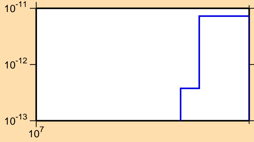
\sigma vs. E for ^{261}\text{Md}(n,\text{He3})
