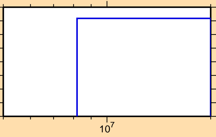
\sigma vs. E for ^{261}\text{Md}(n,np)
