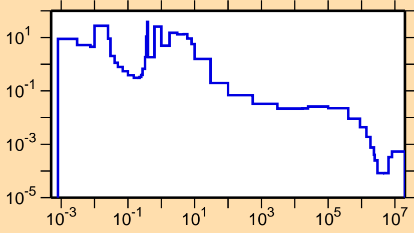
\sigma vs. E for ^{261}\text{Md}(n,\gamma)
